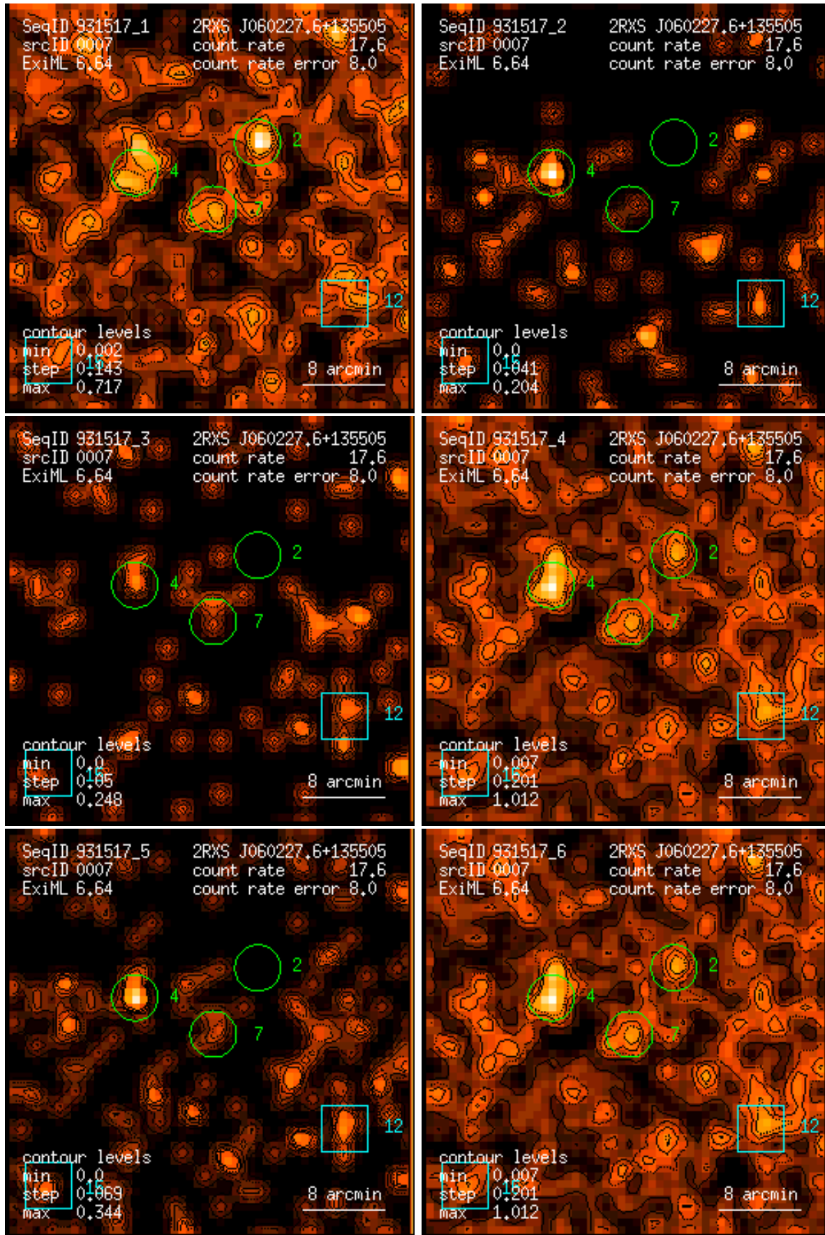
Figure 7: RASS 931517: detection 0007: band rate images, Gaussian filter: (1) PSPC channels 11 – 41, (2) 52 – 90, (3) 91 – 201, (4) 11 – 235, (5) 52 – 201, (6) 11 – 201. Broad band rates in counts/ks. Band rate contour levels in counts/ks/arcmin 2 .
