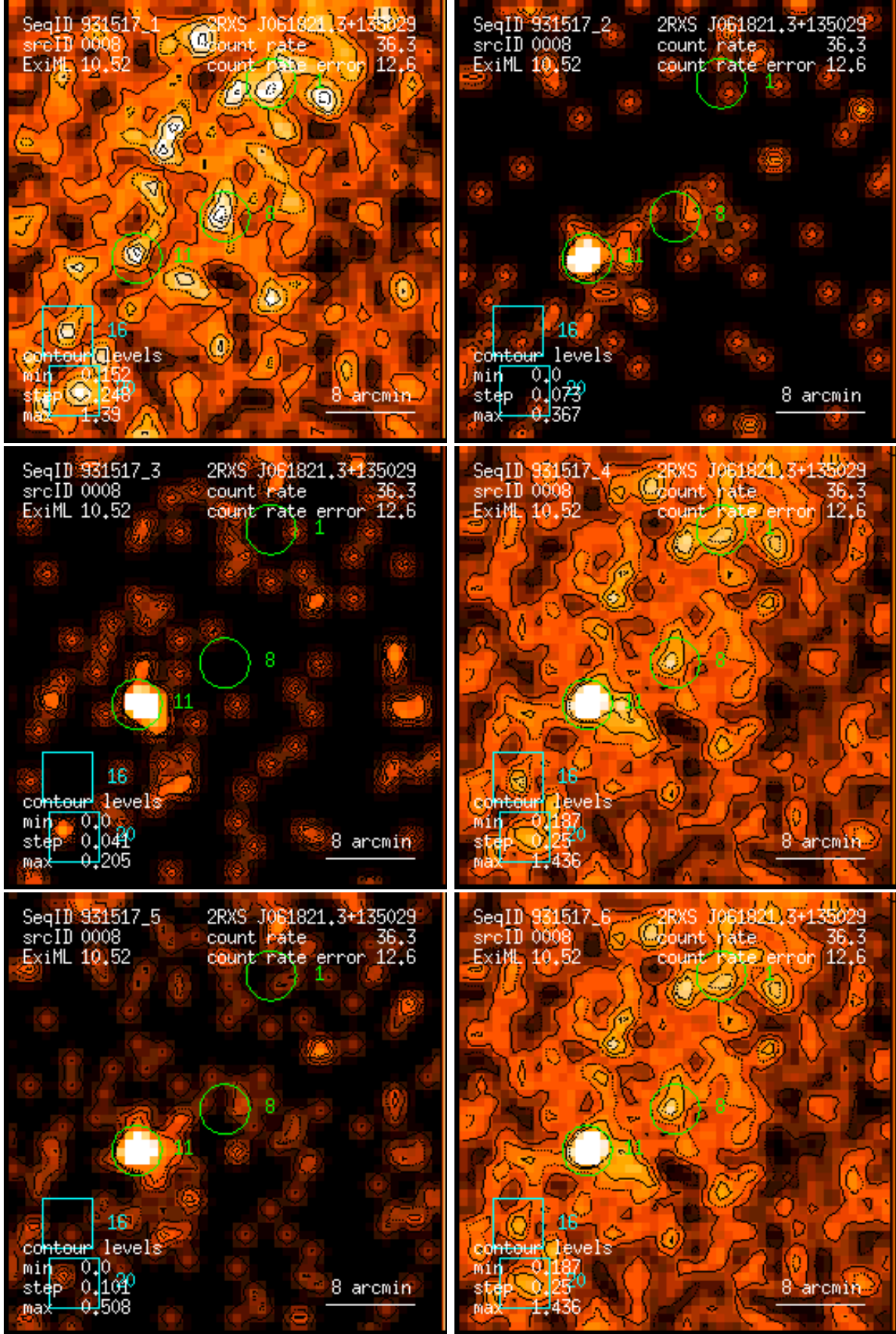
Figure 8: RASS 931517: detection 0008: band rate images, Gaussian filter: (1) PSPC channels 11 – 41, (2) 52 – 90, (3) 91 – 201, (4) 11 – 235, (5) 52 – 201, (6) 11 – 201. Broad band rates in counts/ks. Band rate contour levels in counts/ks/arcmin 2 .
