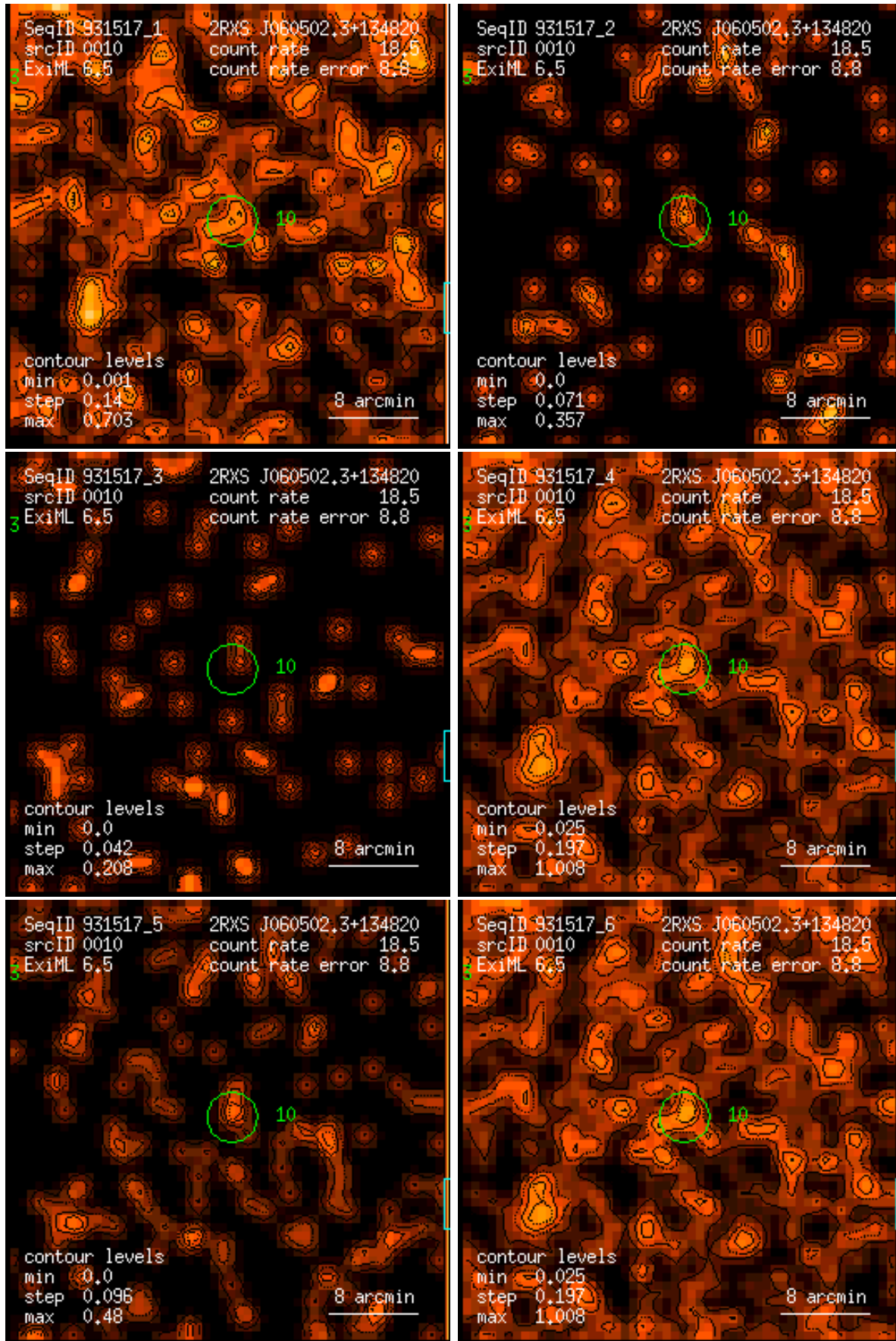
Figure 10: RASS 931517: detection 0010: band rate images, Gaussian filter: (1) PSPC channels 11 – 41, (2) 52 – 90, (3) 91 – 201, (4) 11 – 235, (5) 52 – 201, (6) 11 – 201. Broad band rates in counts/ks. Band rate contour levels in counts/ks/arcmin 2 .
