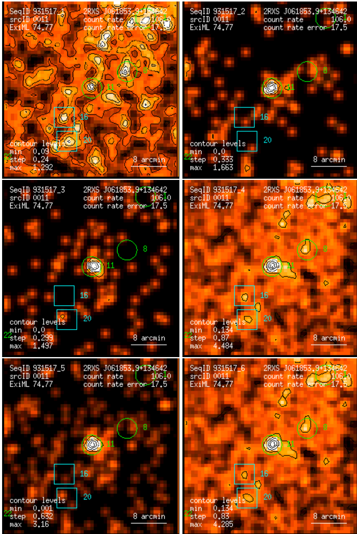
Figure 11: RASS 931517: detection 0011: band rate images, Gaussian filter: (1) PSPC channels 11 – 41, (2) 52 – 90, (3) 91 – 201, (4) 11 – 235, (5) 52 – 201, (6) 11 – 201. Broad band rates in counts/ks. Band rate contour levels in counts/ks/arcmin 2 .
