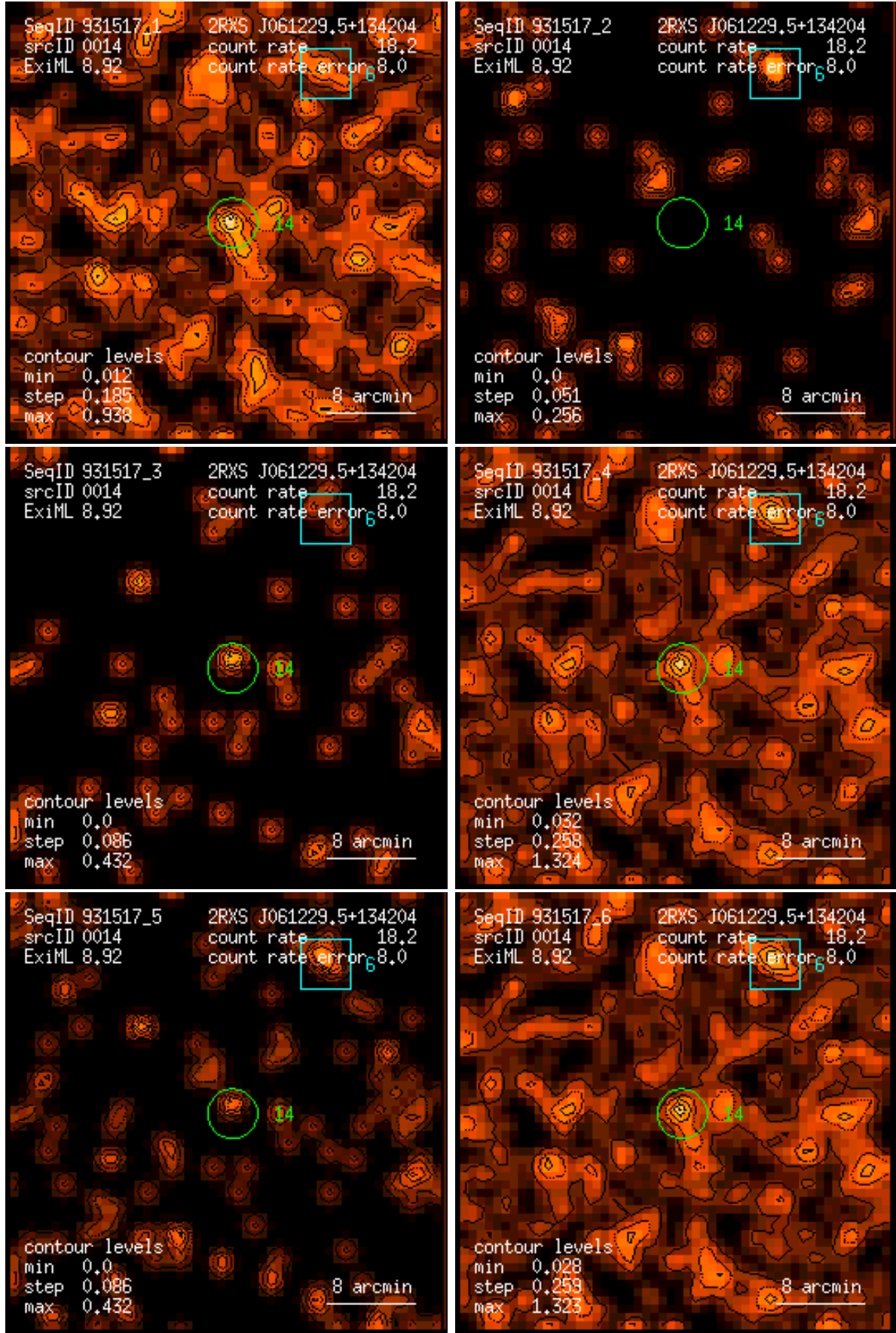
Figure 14: RASS 931517: detection 0014: band rate images, Gaussian filter: (1) PSPC channels 11 – 41, (2) 52 – 90, (3) 91 – 201, (4) 11 – 235, (5) 52 – 201, (6) 11 – 201. Broad band rates in counts/ks. Band rate contour levels in counts/ks/arcmin 2 .
