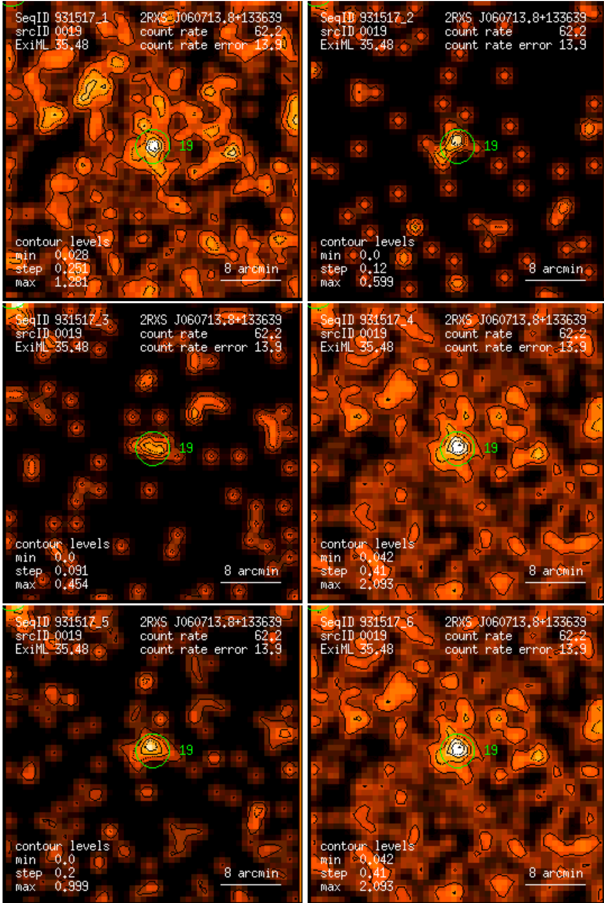
Figure 19: RASS 931517: detection 0019: band rate images, Gaussian filter: (1) PSPC channels 11 – 41, (2) 52 – 90, (3) 91 – 201, (4) 11 – 235, (5) 52 – 201, (6) 11 – 201. Broad band rates in counts/ks. Band rate contour levels in counts/ks/arcmin 2 .
