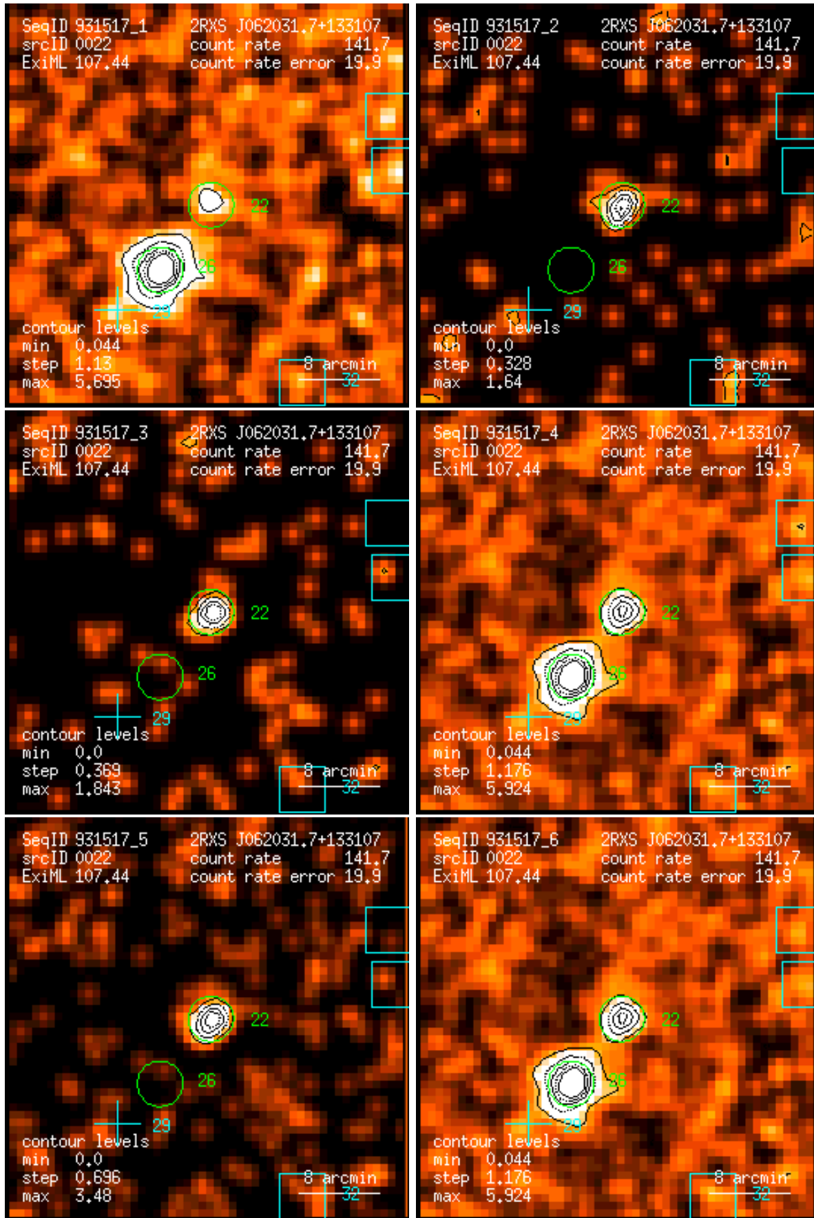
Figure 22: RASS 931517: detection 0022: band rate images, Gaussian filter: (1) PSPC channels 11 – 41, (2) 52 – 90, (3) 91 – 201, (4) 11 – 235, (5) 52 – 201, (6) 11 – 201. Broad band rates in counts/ks. Band rate contour levels in counts/ks/arcmin 2 .
