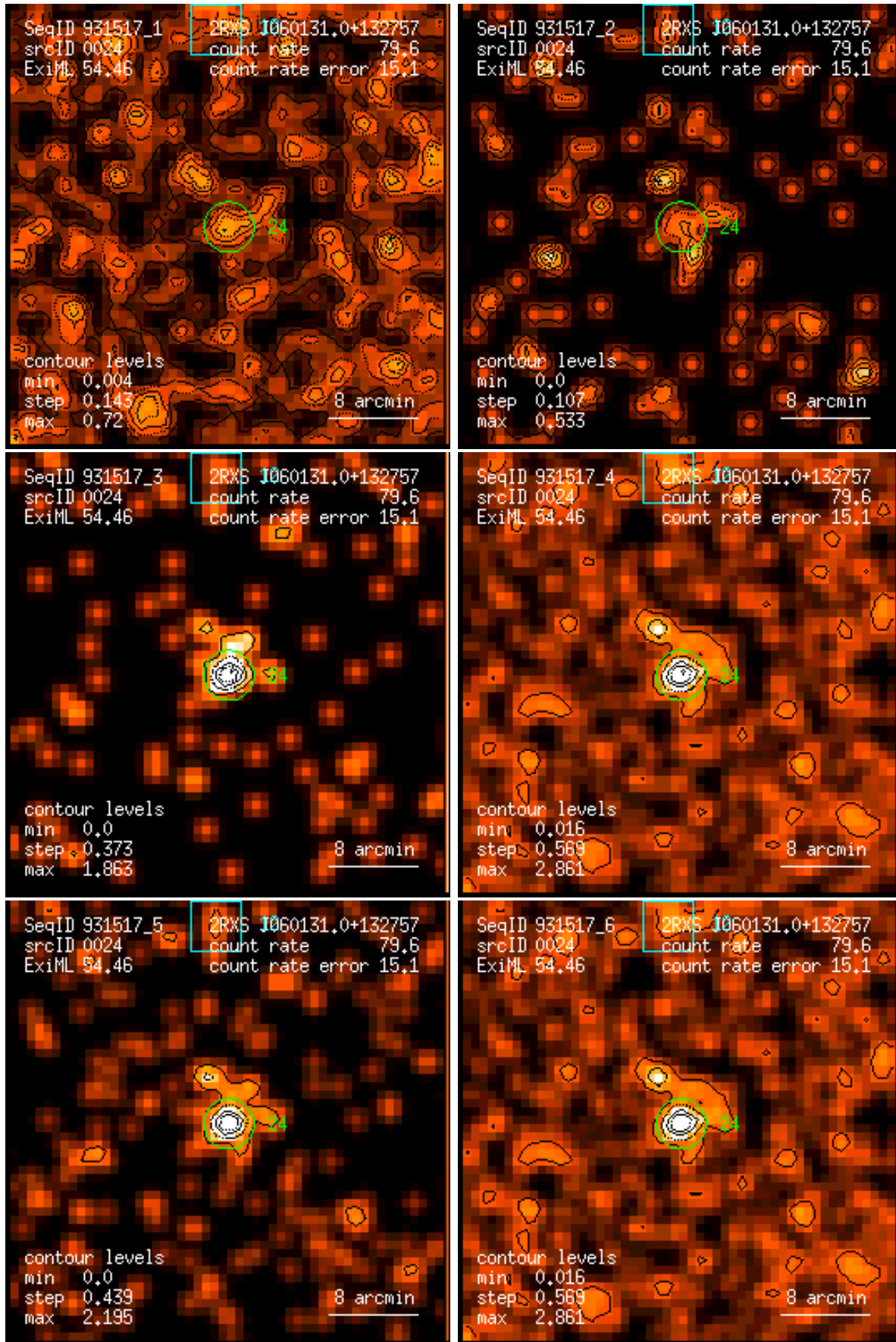
Figure 24: RASS 931517: detection 0024: band rate images, Gaussian filter: (1) PSPC channels 11 – 41, (2) 52 – 90, (3) 91 – 201, (4) 11 – 235, (5) 52 – 201, (6) 11 – 201. Broad band rates in counts/ks. Band rate contour levels in counts/ks/arcmin 2 .
