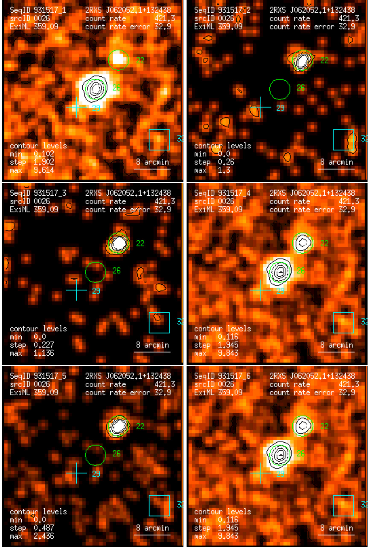
Figure 26: RASS 931517: detection 0026: band rate images, Gaussian filter: (1) PSPC channels 11 – 41, (2) 52 – 90, (3) 91 – 201, (4) 11 – 235, (5) 52 – 201, (6) 11 – 201. Broad band rates in counts/ks. Band rate contour levels in counts/ks/arcmin 2 .
