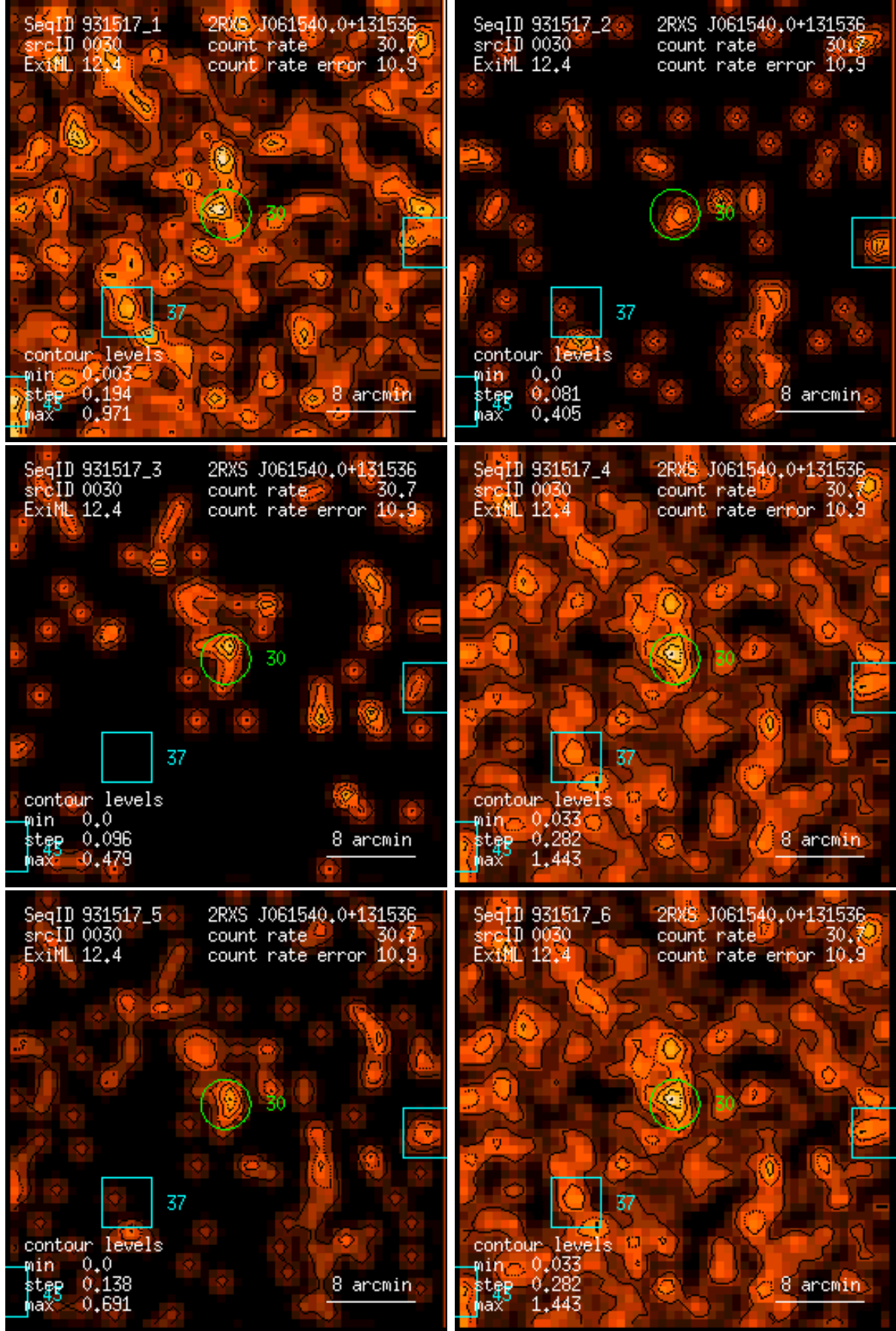
Figure 30: RASS 931517: detection 0030: band rate images, Gaussian filter: (1) PSPC channels 11 – 41, (2) 52 – 90, (3) 91 – 201, (4) 11 – 235, (5) 52 – 201, (6) 11 – 201. Broad band rates in counts/ks. Band rate contour levels in counts/ks/arcmin 2 .
