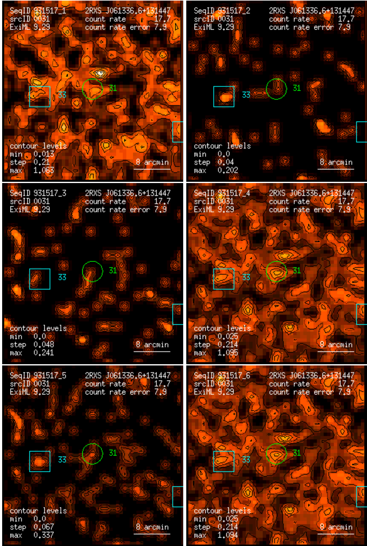
Figure 31: RASS 931517: detection 0031: band rate images, Gaussian filter: (1) PSPC channels 11 – 41, (2) 52 – 90, (3) 91 – 201, (4) 11 – 235, (5) 52 – 201, (6) 11 – 201. Broad band rates in counts/ks. Band rate contour levels in counts/ks/arcmin 2 .
