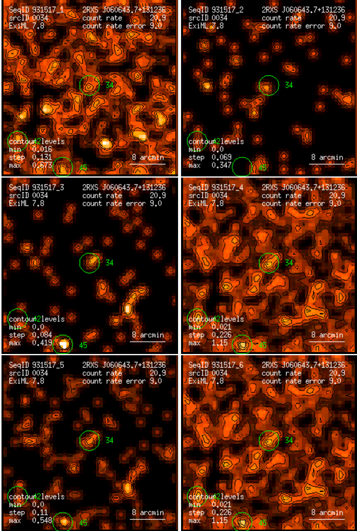
Figure 34: RASS 931517: detection 0034: band rate images, Gaussian filter: (1) PSPC channels 11 – 41, (2) 52 – 90, (3) 91 – 201, (4) 11 – 235, (5) 52 – 201, (6) 11 – 201. Broad band rates in counts/ks. Band rate contour levels in counts/ks/arcmin 2 .
