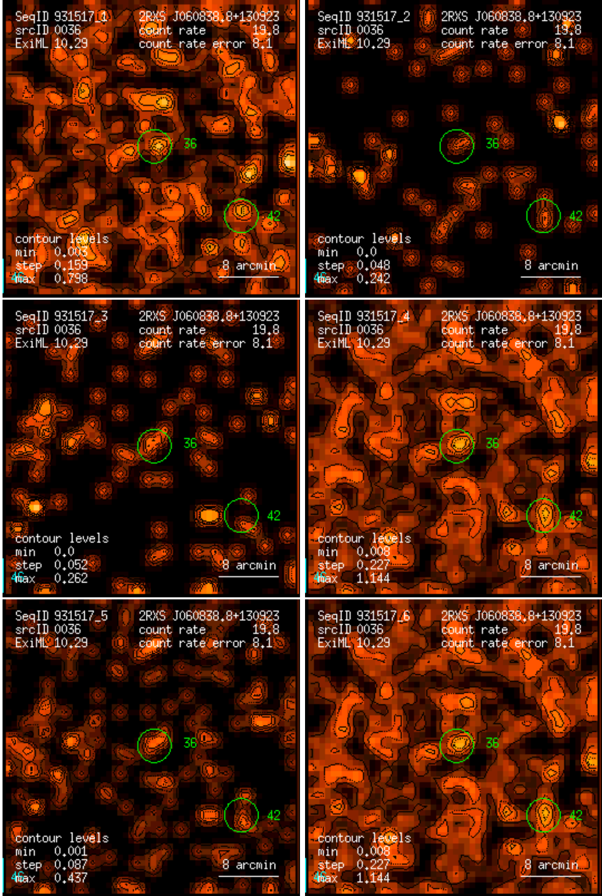
Figure 36: RASS 931517: detection 0036: band rate images, Gaussian filter: (1) PSPC channels 11 – 41, (2) 52 – 90, (3) 91 – 201, (4) 11 – 235, (5) 52 – 201, (6) 11 – 201. Broad band rates in counts/ks. Band rate contour levels in counts/ks/arcmin 2 .
