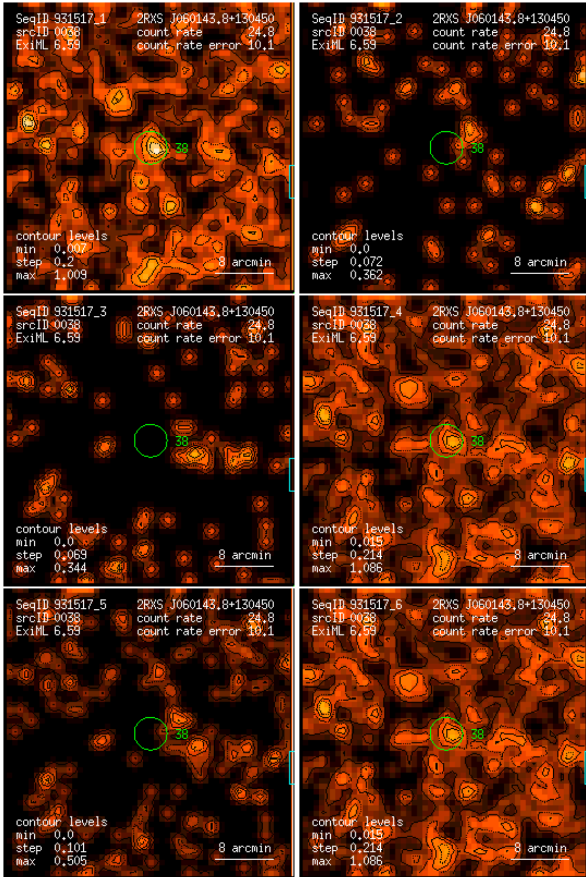
Figure 38: RASS 931517: detection 0038: band rate images, Gaussian filter: (1) PSPC channels 11 – 41, (2) 52 – 90, (3) 91 – 201, (4) 11 – 235, (5) 52 – 201, (6) 11 – 201. Broad band rates in counts/ks. Band rate contour levels in counts/ks/arcmin 2 .
