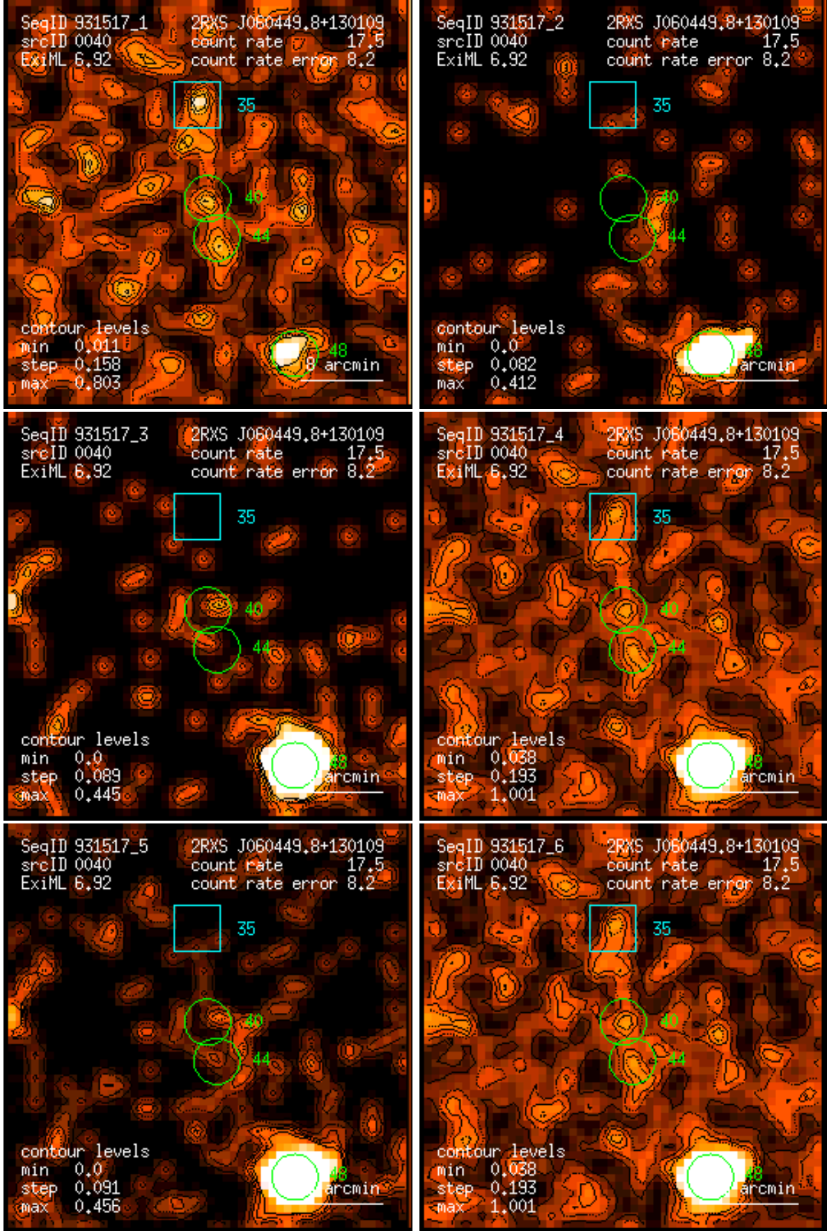
Figure 40: RASS 931517: detection 0040: band rate images, Gaussian filter: (1) PSPC channels 11 – 41, (2) 52 – 90, (3) 91 – 201, (4) 11 – 235, (5) 52 – 201, (6) 11 – 201. Broad band rates in counts/ks. Band rate contour levels in counts/ks/arcmin 2 .
