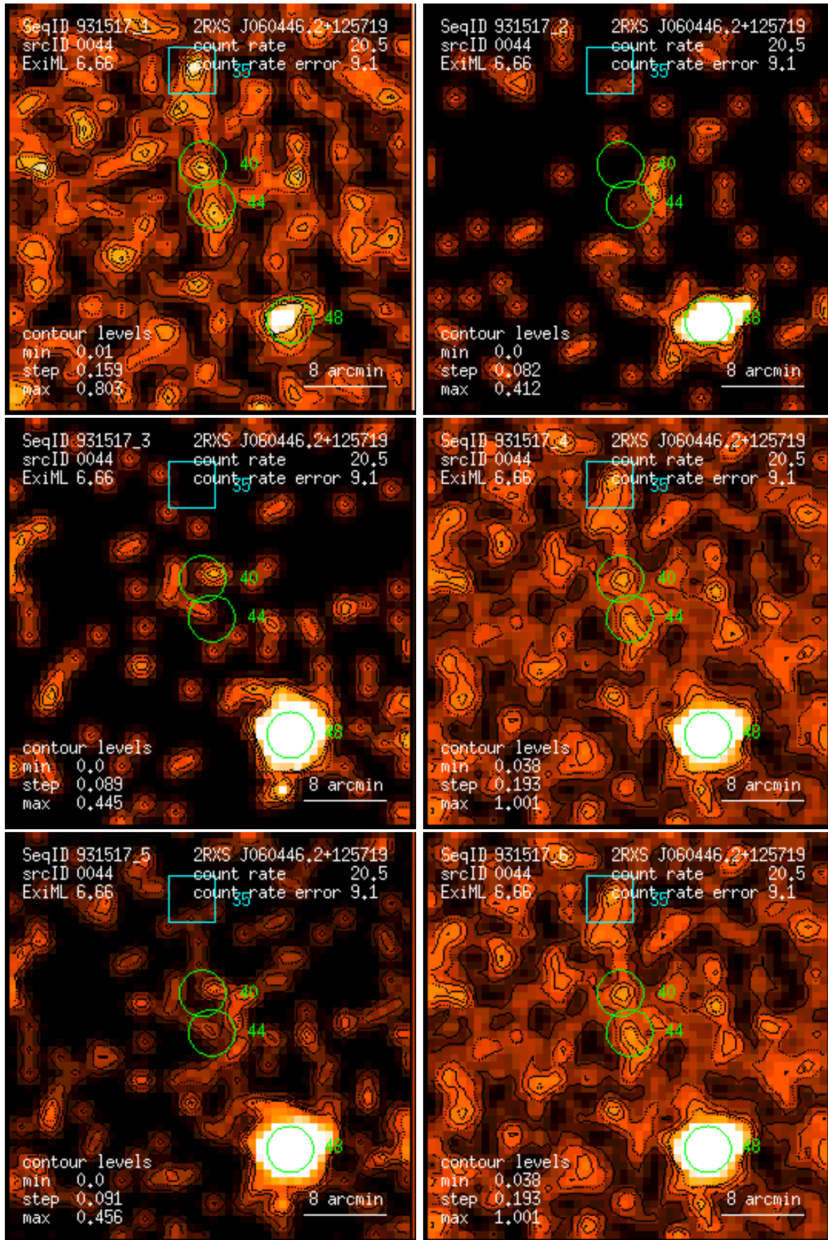
Figure 44: RASS 931517: detection 0044: band rate images, Gaussian filter: (1) PSPC channels 11 – 41, (2) 52 – 90, (3) 91 – 201, (4) 11 – 235, (5) 52 – 201, (6) 11 – 201. Broad band rates in counts/ks. Band rate contour levels in counts/ks/arcmin 2 .
