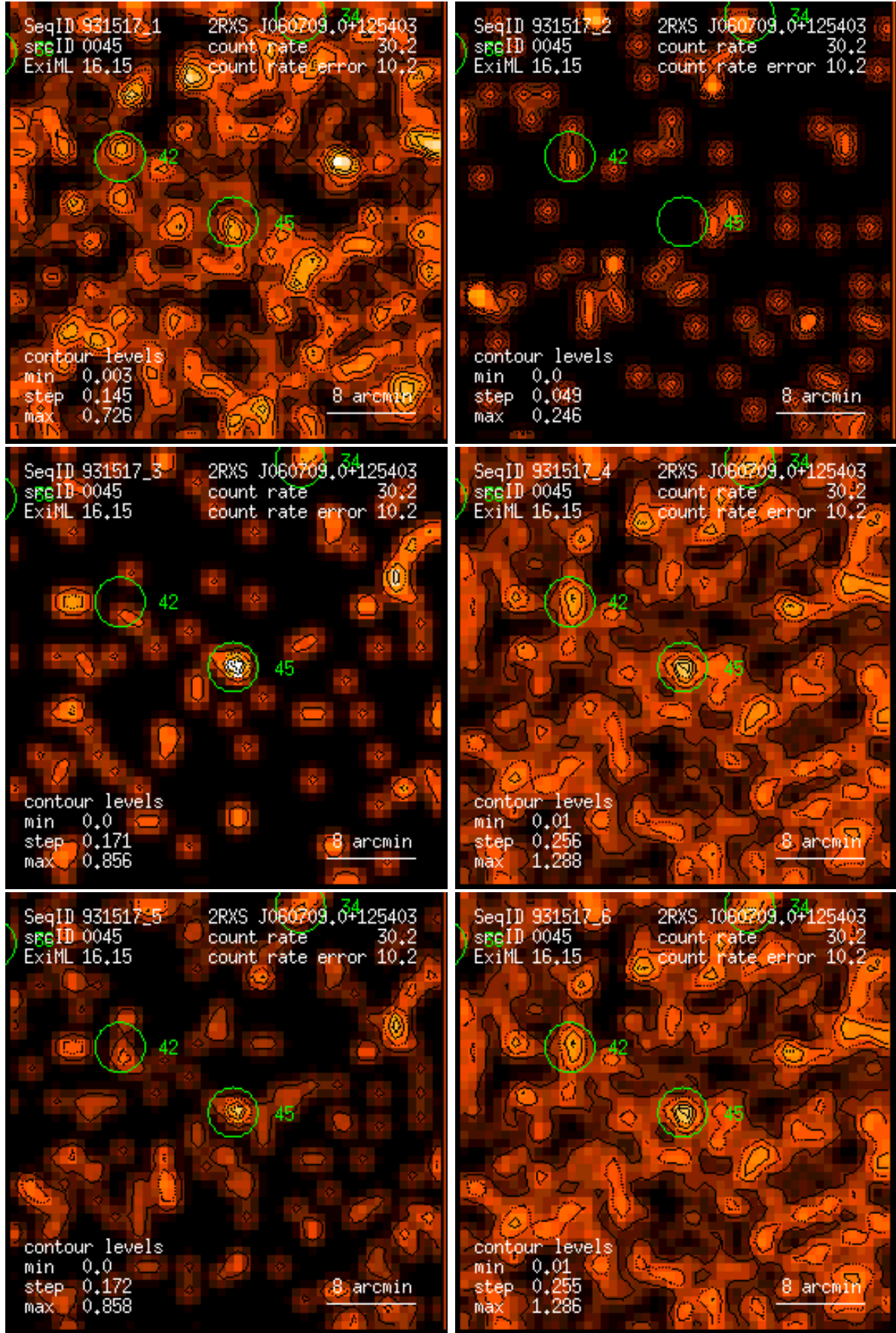
Figure 45: RASS 931517: detection 0045: band rate images, Gaussian filter: (1) PSPC channels 11 – 41, (2) 52 – 90, (3) 91 – 201, (4) 11 – 235, (5) 52 – 201, (6) 11 – 201. Broad band rates in counts/ks. Band rate contour levels in counts/ks/arcmin 2 .
