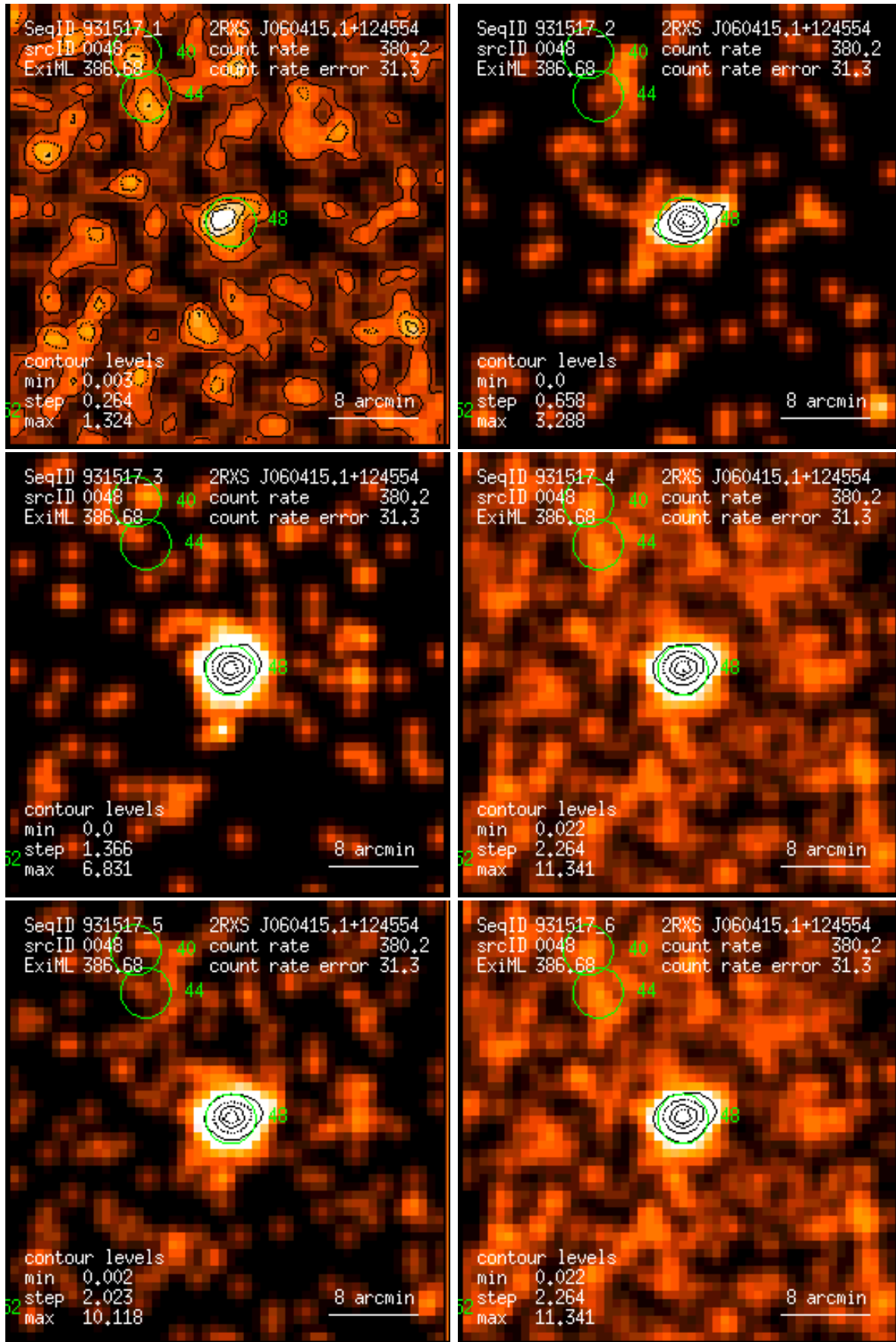
Figure 48: RASS 931517: detection 0048: band rate images, Gaussian filter: (1) PSPC channels 11 – 41, (2) 52 – 90, (3) 91 – 201, (4) 11 – 235, (5) 52 – 201, (6) 11 – 201. Broad band rates in counts/ks. Band rate contour levels in counts/ks/arcmin 2 .
