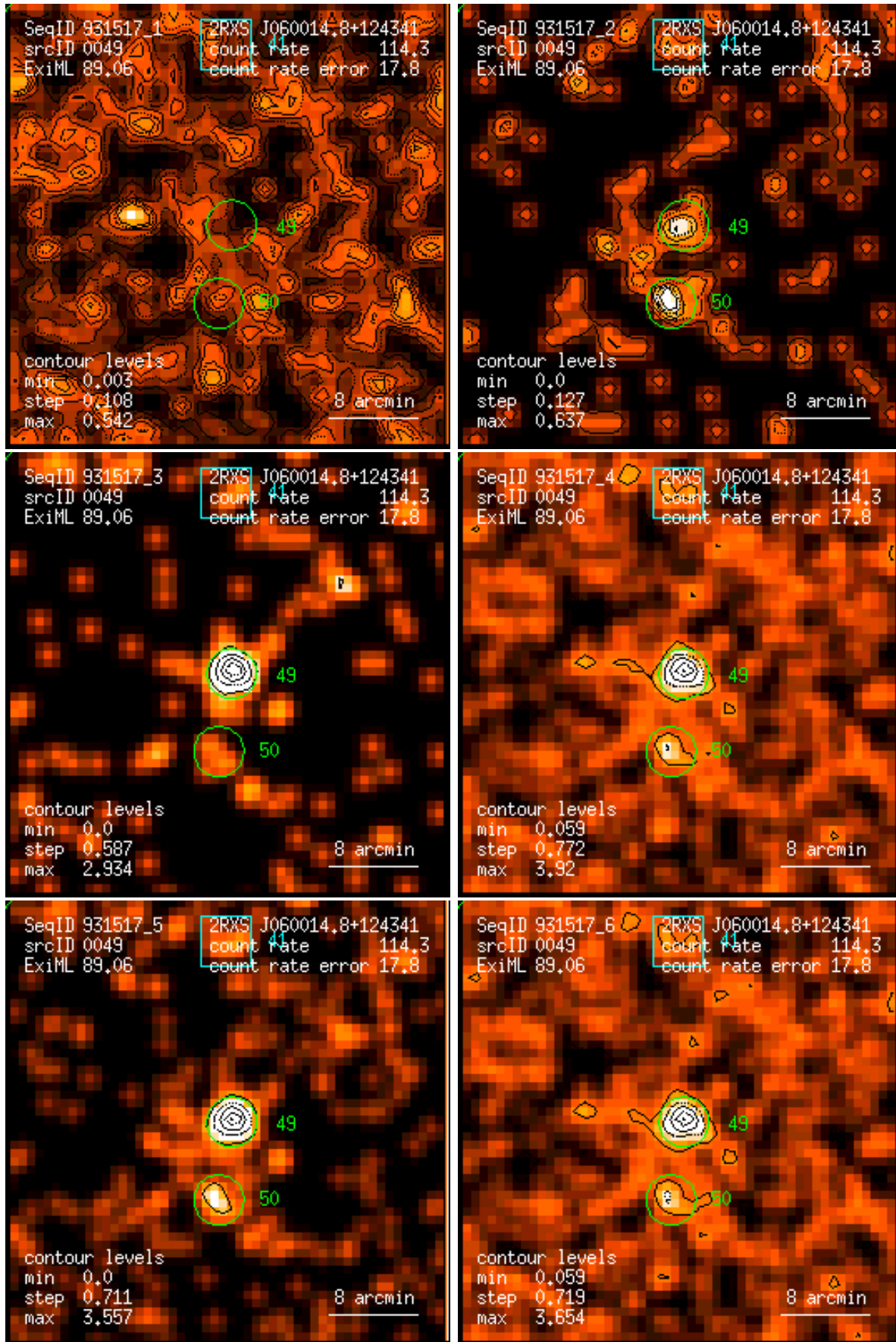
Figure 49: RASS 931517: detection 0049: band rate images, Gaussian filter: (1) PSPC channels 11 – 41, (2) 52 – 90, (3) 91 – 201, (4) 11 – 235, (5) 52 – 201, (6) 11 – 201. Broad band rates in counts/ks. Band rate contour levels in counts/ks/arcmin 2 .
