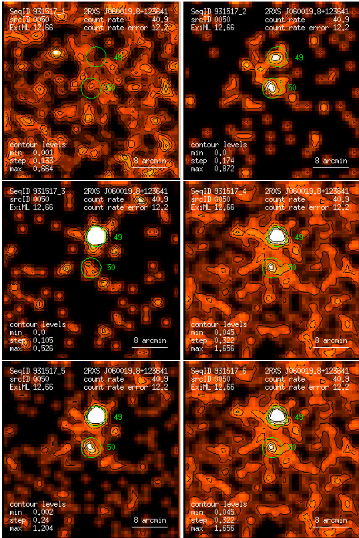
Figure 50: RASS 931517: detection 0050: band rate images, Gaussian filter: (1) PSPP channels 11 – 41, (2) 52 – 90, (3) 91 – 201, (4) 11 – 235, (5) 52 – 201, (6) 11 – 201. Broad band rates in counts/ks. Band rate contour levels in counts/ks/arcmin 2 .
