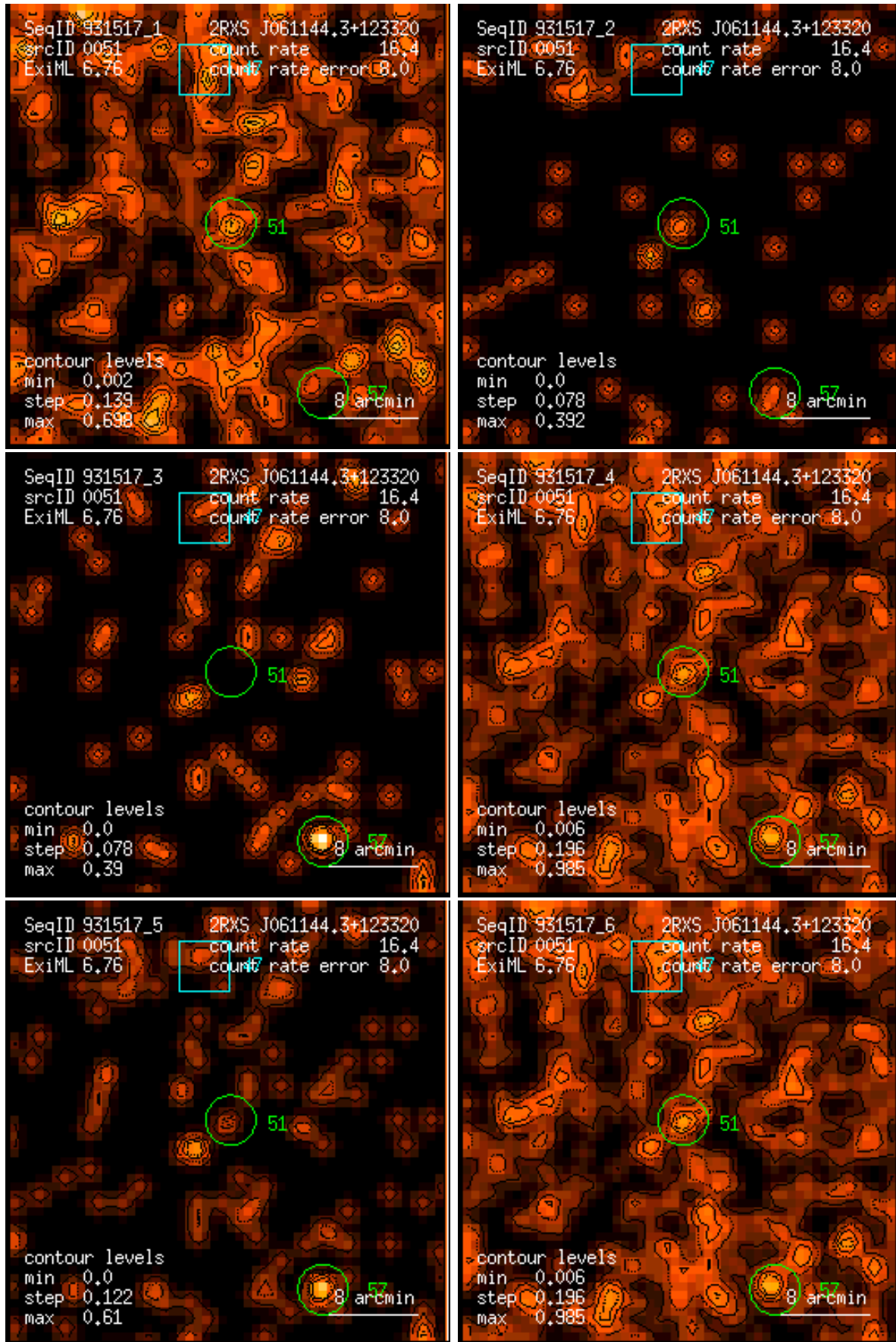
Figure 51: RASS 931517: detection 0051: band rate images, Gaussian filter: (1) PSPC channels 11 – 41, (2) 52 – 90, (3) 91 – 201, (4) 11 – 235, (5) 52 – 201, (6) 11 – 201. Broad band rates in counts/ks. Band rate contour levels in counts/ks/arcmin 2 .
