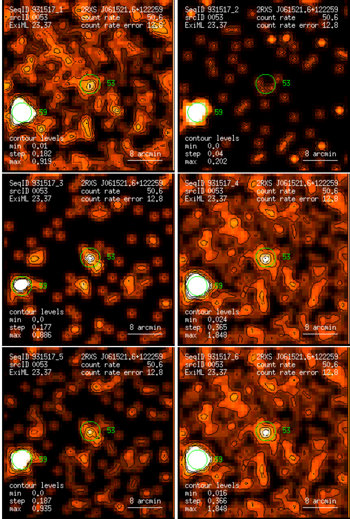
Figure 53: RASS 931517: detection 0053: band rate images, Gaussian filter: (1) PSPC channels 11 – 41, (2) 52 – 90, (3) 91 – 201, (4) 11 – 235, (5) 52 – 201, (6) 11 – 201. Broad band rates in counts/ks. Band rate contour levels in counts/ks/arcmin 2 .
