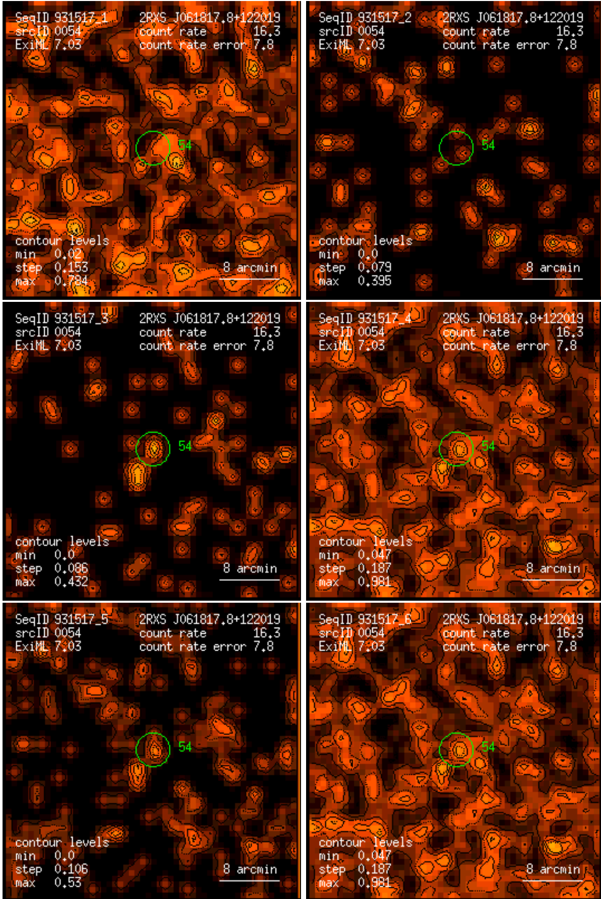
Figure 54: RASS 931517: detection 0054: band rate images, Gaussian filter: (1) PSPC channels 11 – 41, (2) 52 – 90, (3) 91 – 201, (4) 11 – 235, (5) 52 – 201, (6) 11 – 201. Broad band rates in counts/ks. Band rate contour levels in counts/ks/arcmin 2 .
