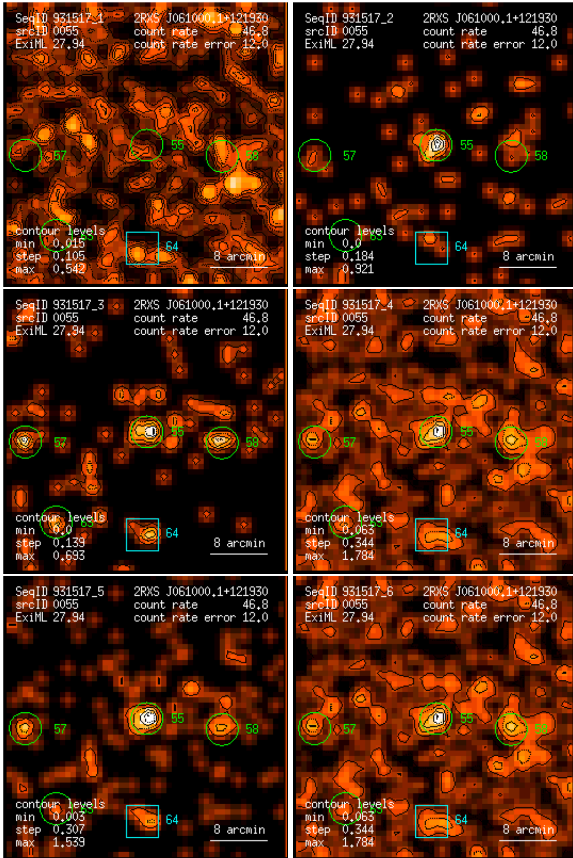
Figure 55: RASS 931517: detection 0055: band rate images, Gaussian filter: (1) PSPC channels 11 – 41, (2) 52 – 90, (3) 91 – 201, (4) 11 – 235, (5) 52 – 201, (6) 11 – 201. Broad band rates in counts/ks. Band rate contour levels in counts/ks/arcmin 2 .
