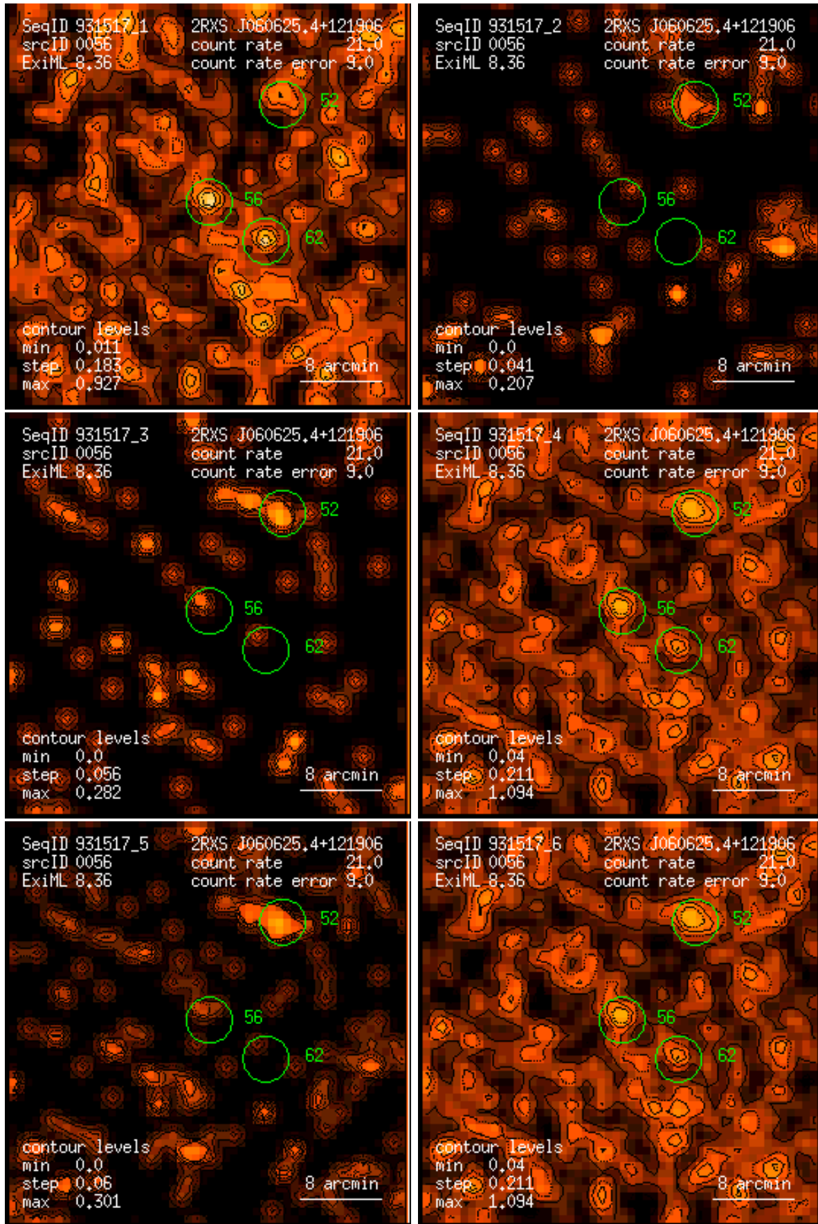
Figure 56: RASS 931517: detection 0056: band rate images, Gaussian filter: (1) PSPC channels 11 – 41, (2) 52 – 90, (3) 91 – 201, (4) 11 – 235, (5) 52 – 201, (6) 11 – 201. Broad band rates in counts/ks. Band rate contour levels in counts/ks/arcmin 2 .
