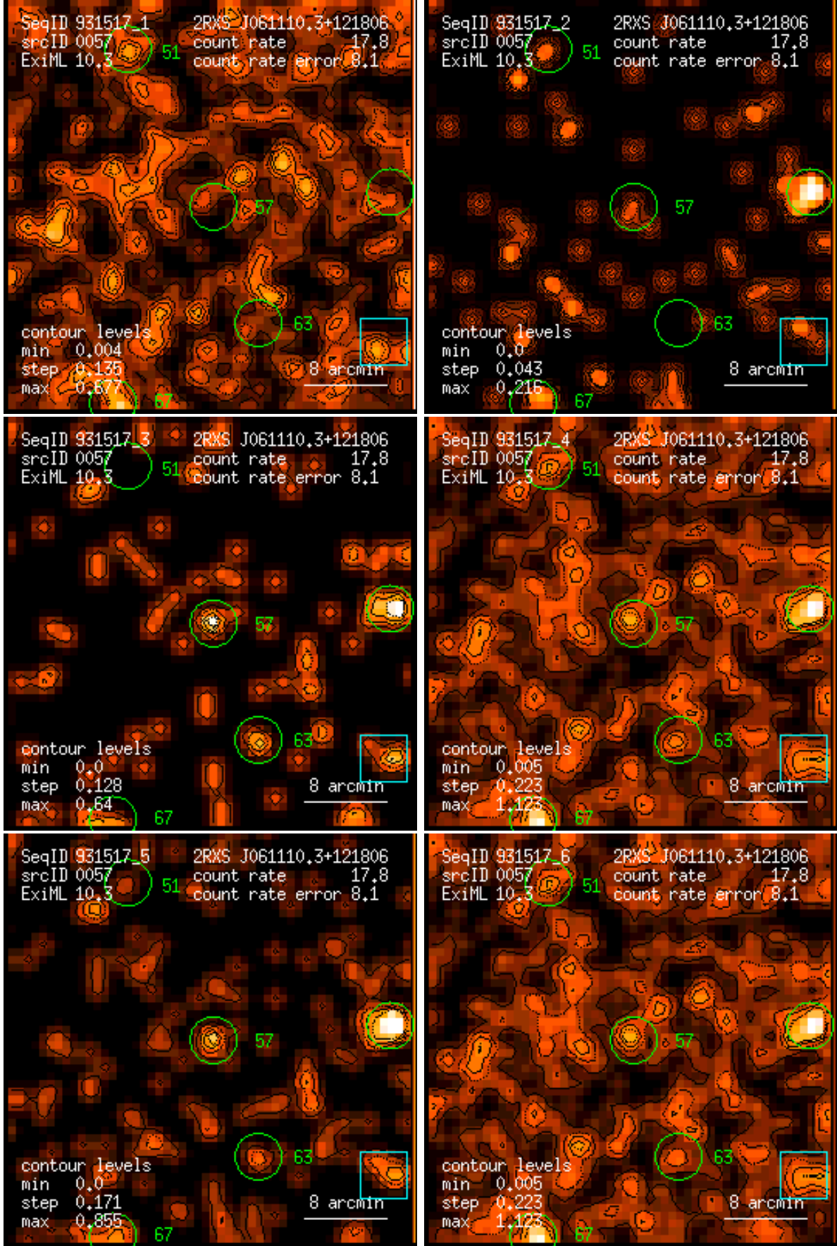
Figure 57: RASS 931517: detection 0057: band rate images, Gaussian filter: (1) PSPC channels 11 – 41, (2) 52 – 90, (3) 91 – 201, (4) 11 – 235, (5) 52 – 201, (6) 11 – 201. Broad band rates in counts/ks. Band rate contour levels in counts/ks/arcmin 2 .
