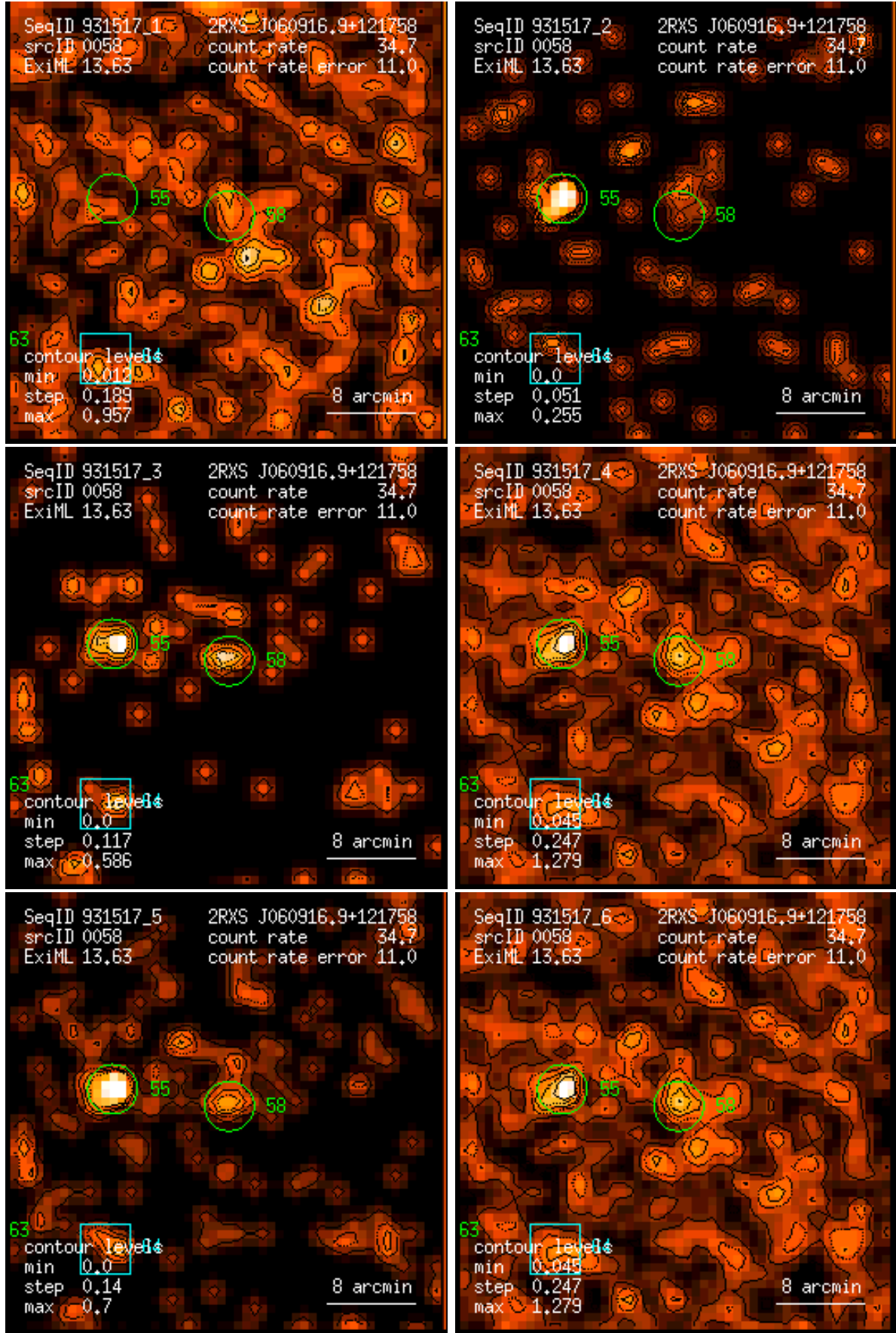
Figure 58: RASS 931517: detection 0058: band rate images, Gaussian filter: (1) PSPC channels 11 – 41, (2) 52 – 90, (3) 91 – 201, (4) 11 – 235, (5) 52 – 201, (6) 11 – 201. Broad band rates in counts/ks. Band rate contour levels in counts/ks/arcmin 2 .
