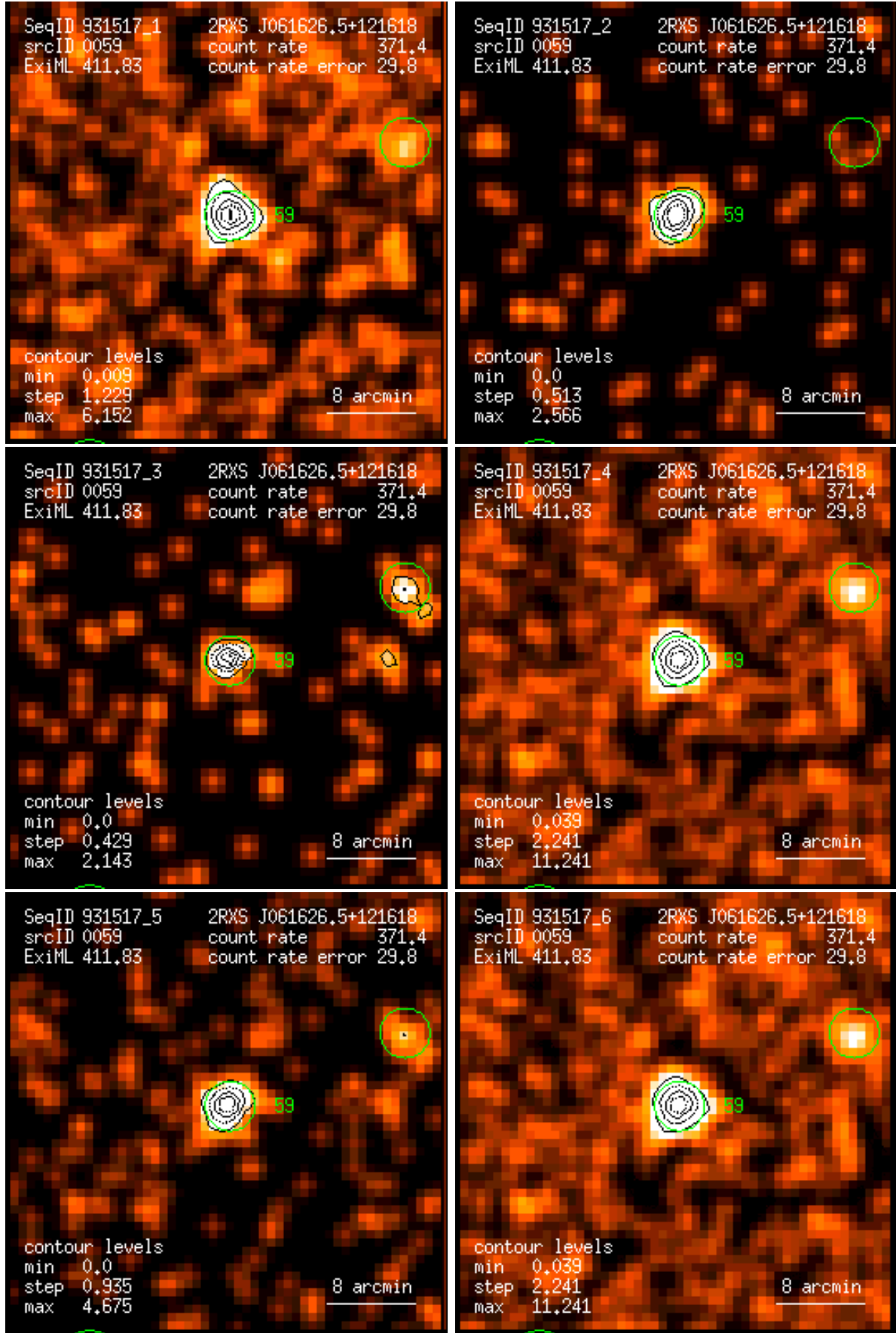
Figure 59: RASS 931517: detection 0059: band rate images, Gaussian filter: (1) PSPC channels 11 – 41, (2) 52 – 90, (3) 91 – 201, (4) 11 – 235, (5) 52 – 201, (6) 11 – 201. Broad band rates in counts/ks. Band rate contour levels in counts/ks/arcmin 2 .
