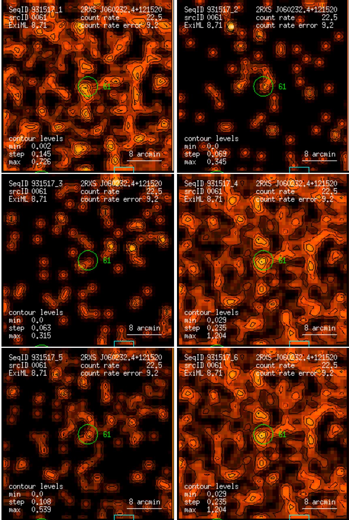
Figure 61: RASS 931517: detection 0061: band rate images, Gaussian filter: (1) PSPC channels 11 – 41, (2) 52 – 90, (3) 91 – 201, (4) 11 – 235, (5) 52 – 201, (6) 11 – 201. Broad band rates in counts/ks. Band rate contour levels in counts/ks/arcmin 2 .
