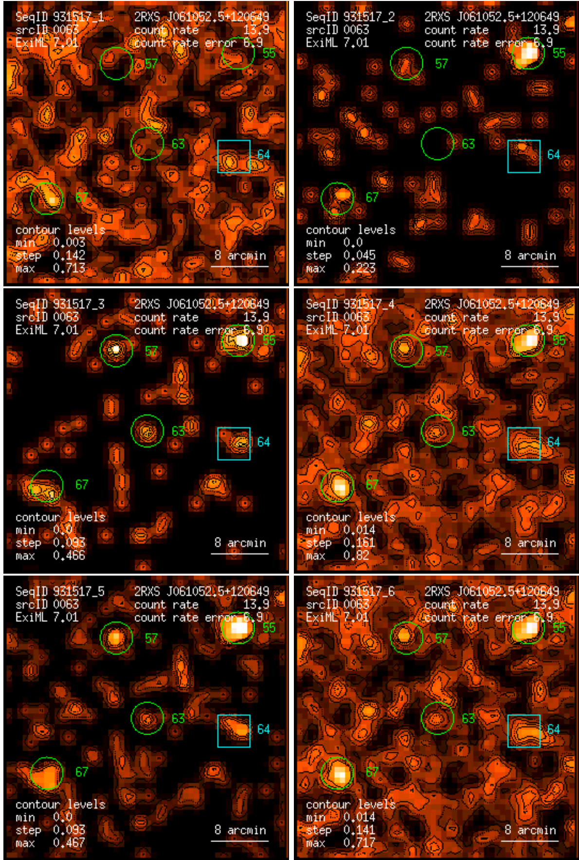
Figure 63: RASS 931517: detection 0063: band rate images, Gaussian filter: (1) PSPC channels 11 – 41, (2) 52 – 90, (3) 91 – 201, (4) 11 – 235, (5) 52 – 201, (6) 11 – 201. Broad band rates in counts/ks. Band rate contour levels in counts/ks/arcmin 2 .
