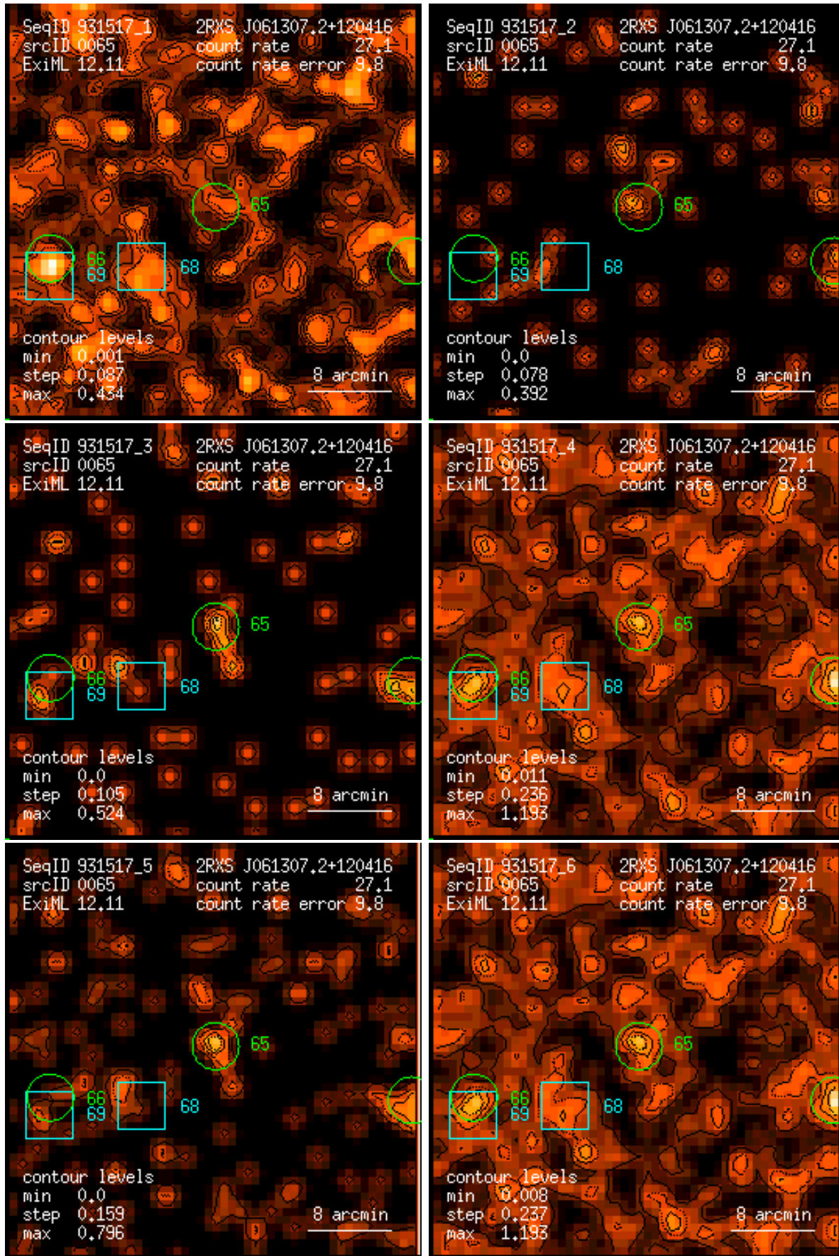
Figure 65: RASS 931517: detection 0065: band rate images, Gaussian filter: (1) PSPC channels 11 – 41, (2) 52 – 90, (3) 91 – 201, (4) 11 – 235, (5) 52 – 201, (6) 11 – 201. Broad band rates in counts/ks. Band rate contour levels in counts/ks/arcmin 2 .
