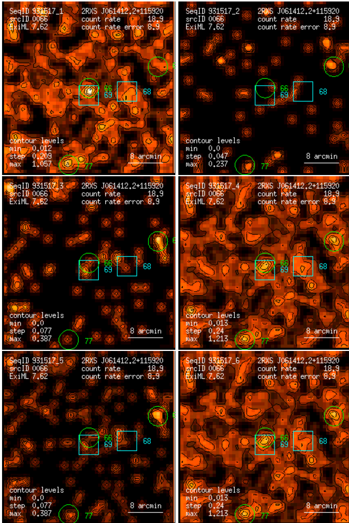
Figure 66: RASS 931517: detection 0066: band rate images, Gaussian filter: (1) PSPC channels 11 – 41, (2) 52 – 90, (3) 91 – 201, (4) 11 – 235, (5) 52 – 201, (6) 11 – 201. Broad band rates in counts/ks. Band rate contour levels in counts/ks/arcmin 2 .
