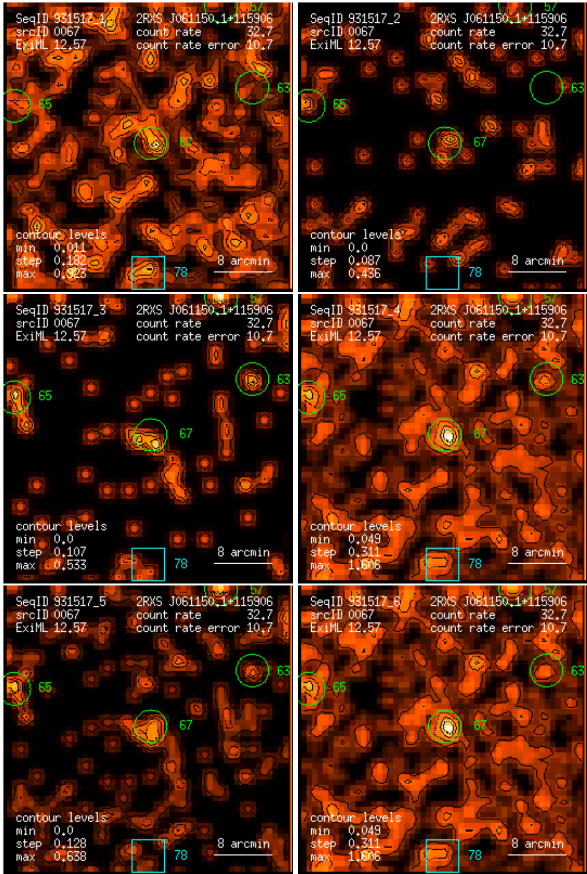
Figure 67: RASS 931517: detection 0067: band rate images, Gaussian filter: (1) PSPC channels 11 – 41, (2) 52 – 90, (3) 91 – 201, (4) 11 – 235, (5) 52 – 201, (6) 11 – 201. Broad band rates in counts/ks. Band rate contour levels in counts/ks/arcmin 2 .
