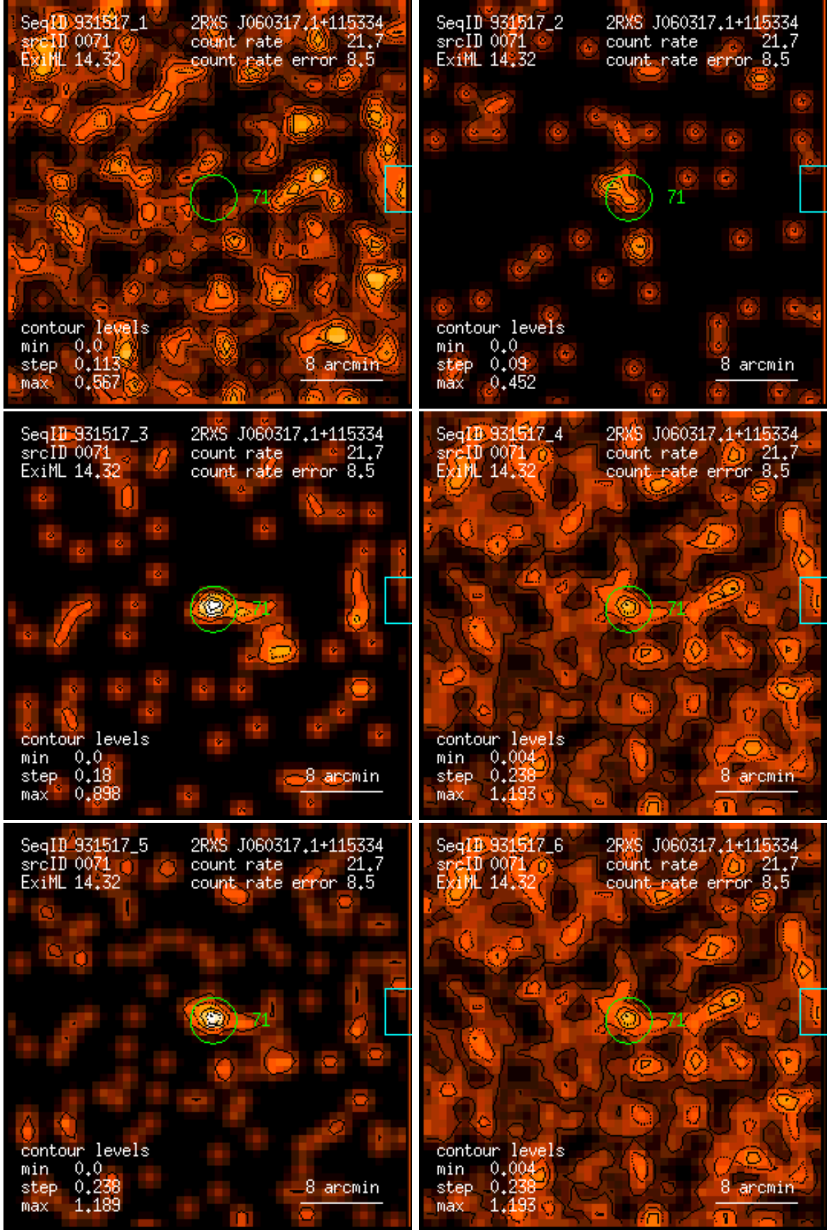
Figure 71: RASS 931517: detection 0071: band rate images, Gaussian filter: (1) PSPC channels 11 – 41, (2) 52 – 90, (3) 91 – 201, (4) 11 – 235, (5) 52 – 201, (6) 11 – 201. Broad band rates in counts/ks. Band rate contour levels in counts/ks/arcmin 2 .
