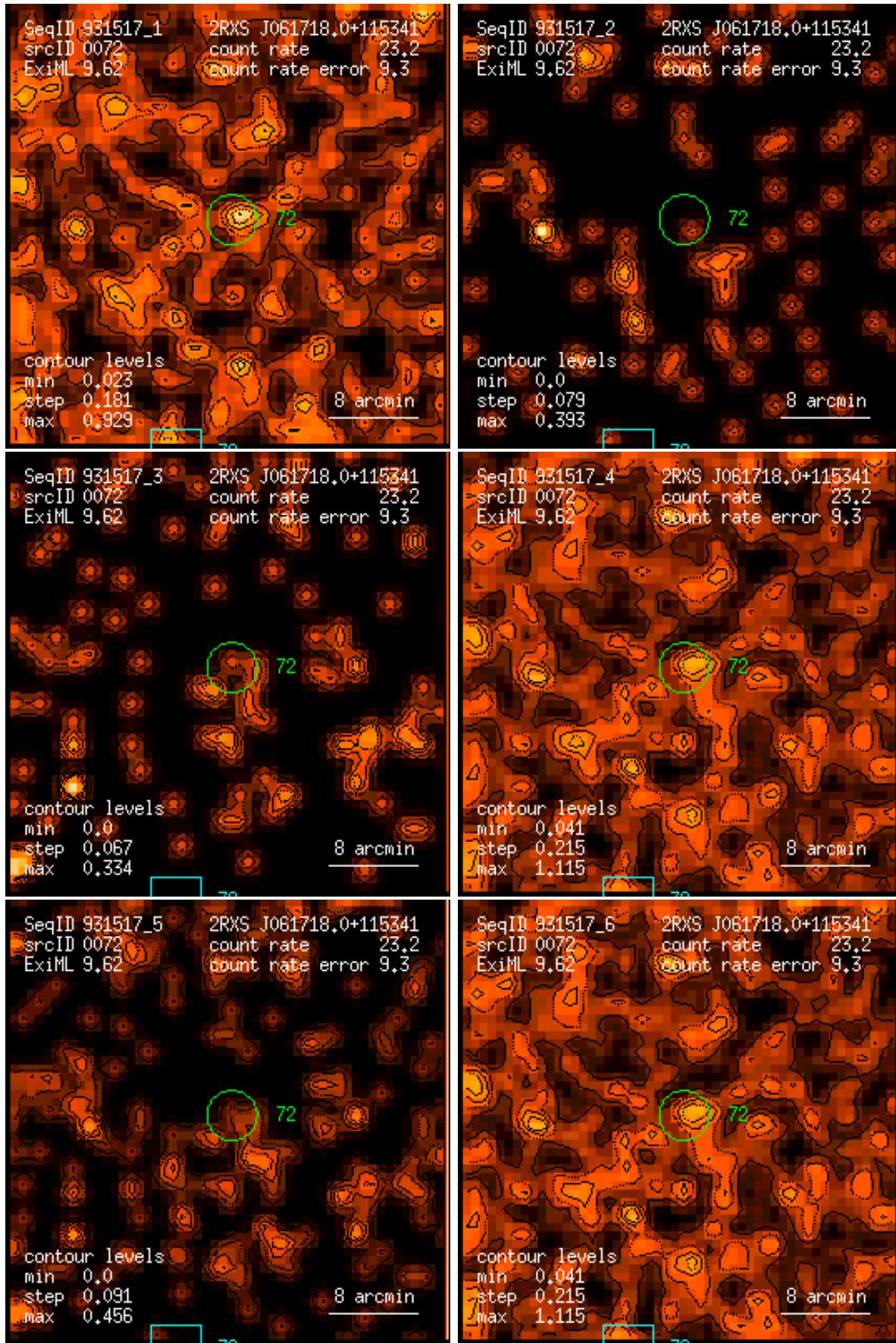
Figure 72: RASS 931517: detection 0072: band rate images, Gaussian filter: (1) PSPC channels 11 – 41, (2) 52 – 90, (3) 91 – 201, (4) 11 – 235, (5) 52 – 201, (6) 11 – 201. Broad band rates in counts/ks. Band rate contour levels in counts/ks/arcmin 2 .
