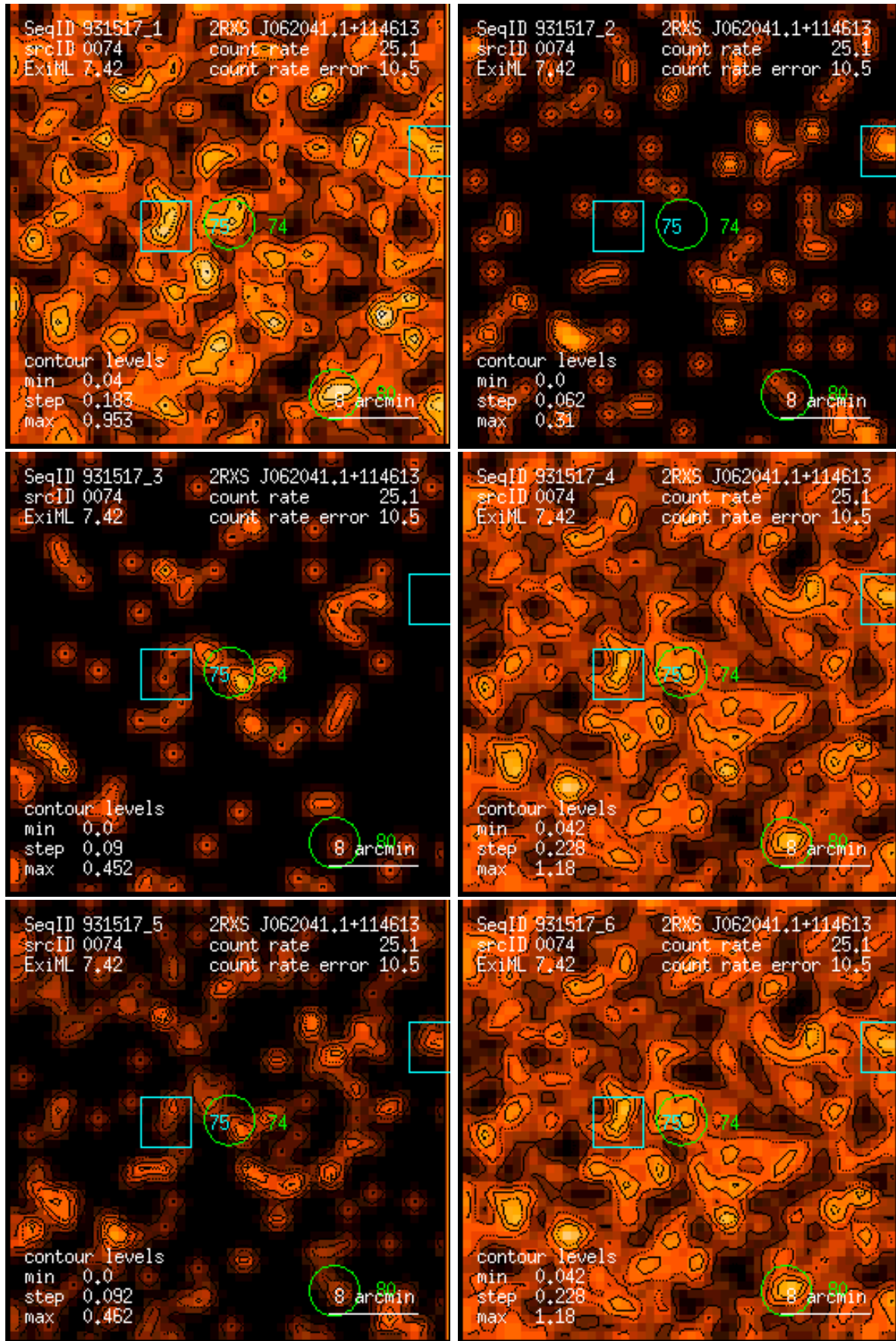
Figure 74: RASS 931517: detection 0074: band rate images, Gaussian filter: (1) PSPC channels 11 – 41, (2) 52 – 90, (3) 91 – 201, (4) 11 – 235, (5) 52 – 201, (6) 11 – 201. Broad band rates in counts/ks. Band rate contour levels in counts/ks/arcmin 2 .
