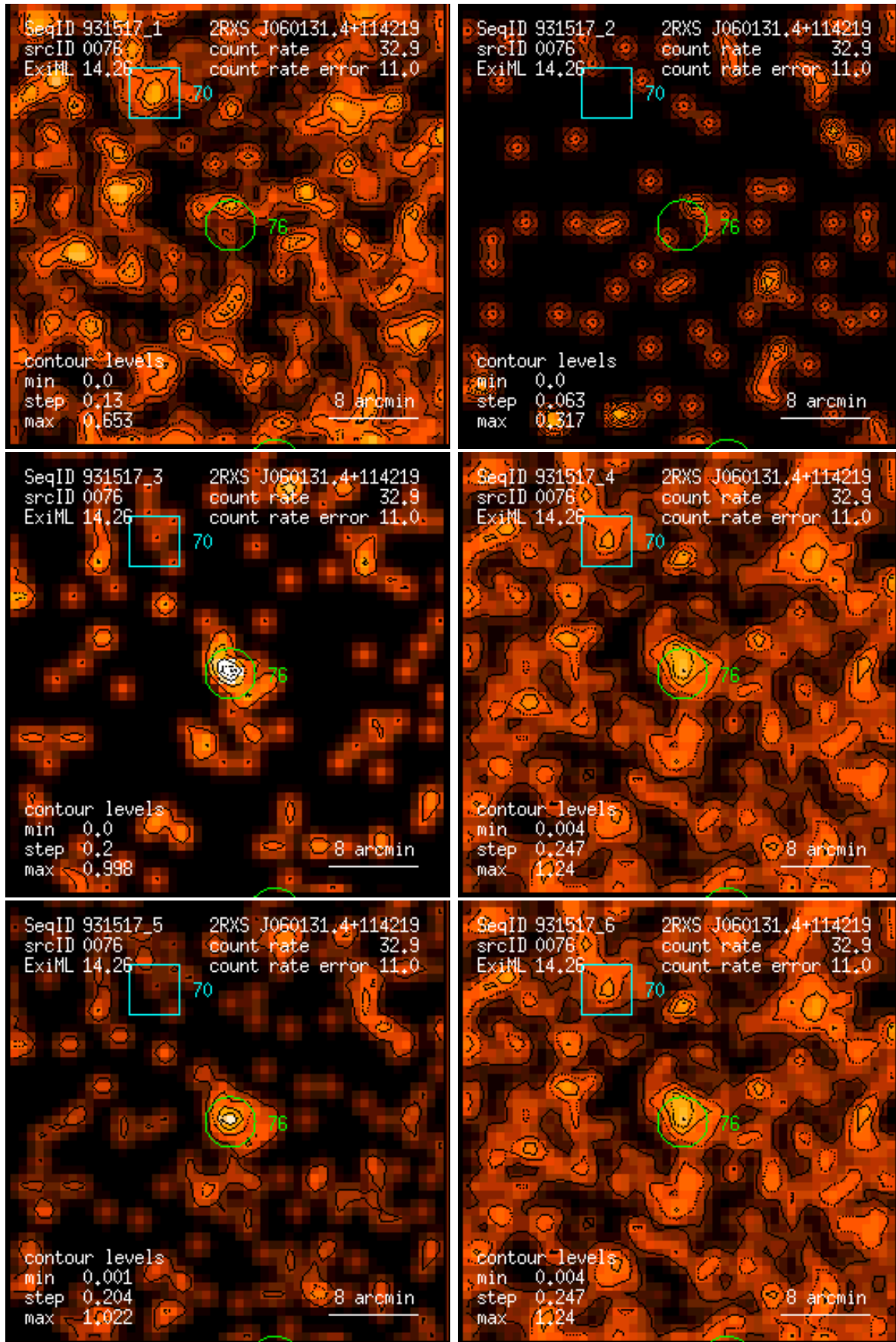
Figure 76: RASS 931517: detection 0076: band rate images, Gaussian filter: (1) PSPC channels 11 – 41, (2) 52 – 90, (3) 91 – 201, (4) 11 – 235, (5) 52 – 201, (6) 11 – 201. Broad band rates in counts/ks. Band rate contour levels in counts/ks/arcmin 2 .
