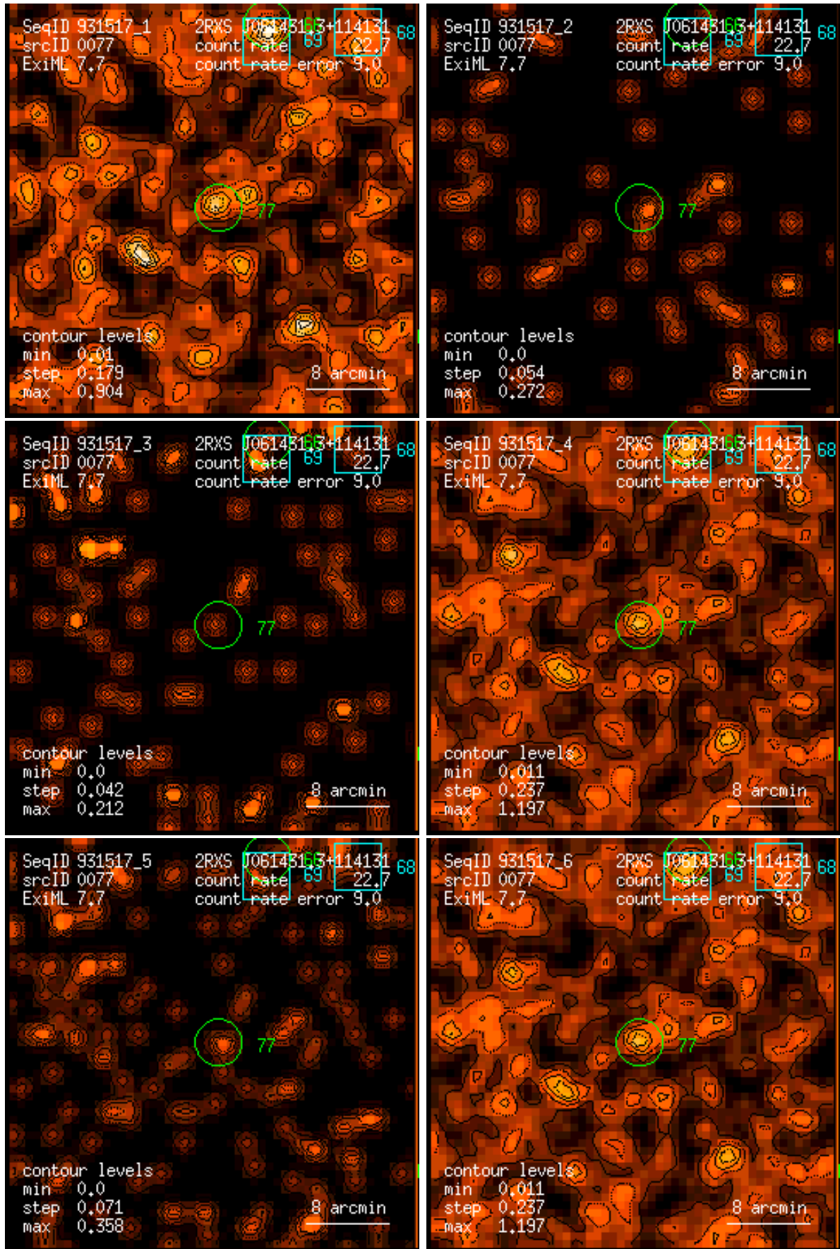
Figure 77: RASS 931517: detection 0077: band rate images, Gaussian filter: (1) PSPC channels 11 – 41, (2) 52 – 90, (3) 91 – 201, (4) 11 – 235, (5) 52 – 201, (6) 11 – 201. Broad band rates in counts/ks. Band rate contour levels in counts/ks/arcmin 2 .
