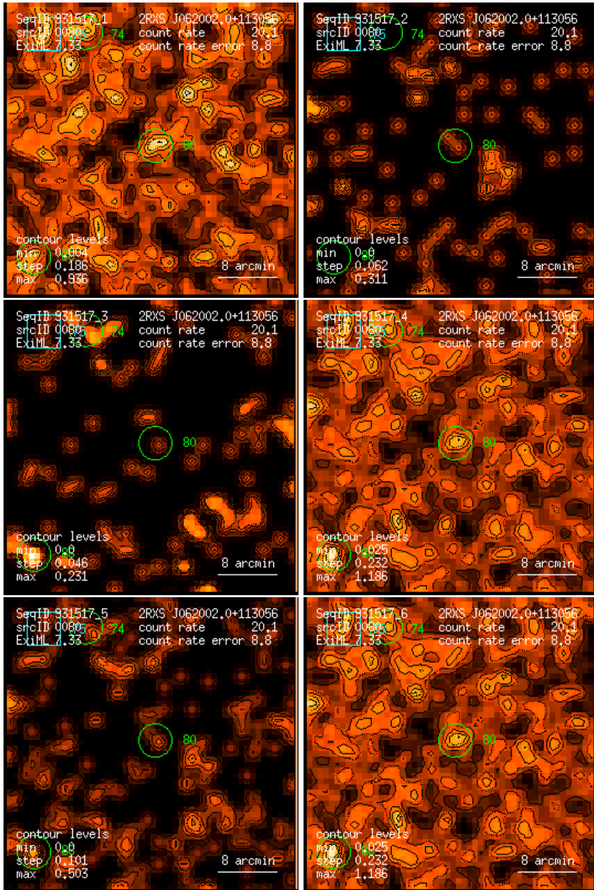
Figure 80: RASS 931517: detection 0080: band rate images, Gaussian filter: (1) PSPC channels 11 – 41, (2) 52 – 90, (3) 91 – 201, (4) 11 – 235, (5) 52 – 201, (6) 11 – 201. Broad band rates in counts/ks. Band rate contour levels in counts/ks/arcmin 2 .
