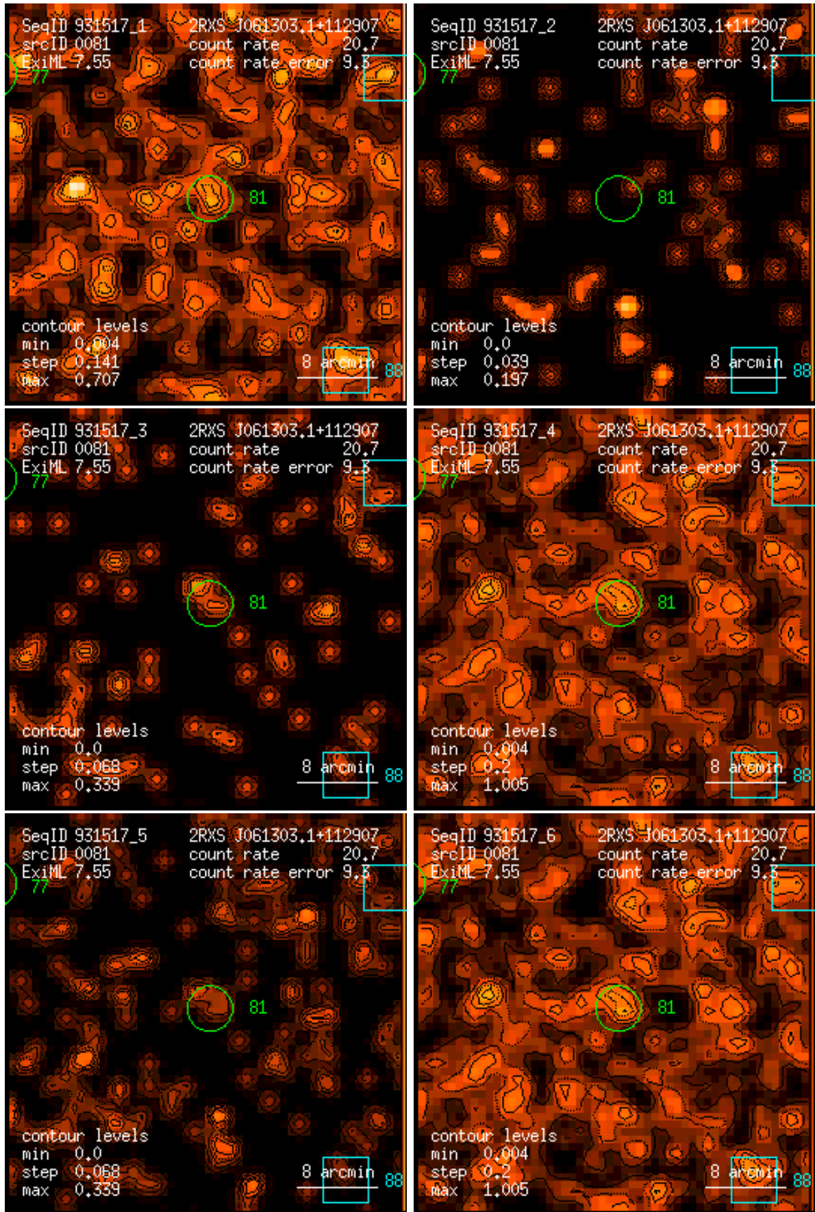
Figure 81: RASS 931517: detection 0081: band rate images, Gaussian filter: (1) PSPC channels 11 – 41, (2) 52 – 90, (3) 91 – 201, (4) 11 – 235, (5) 52 – 201, (6) 11 – 201. Broad band rates in counts/ks. Band rate contour levels in counts/ks/arcmin 2 .
