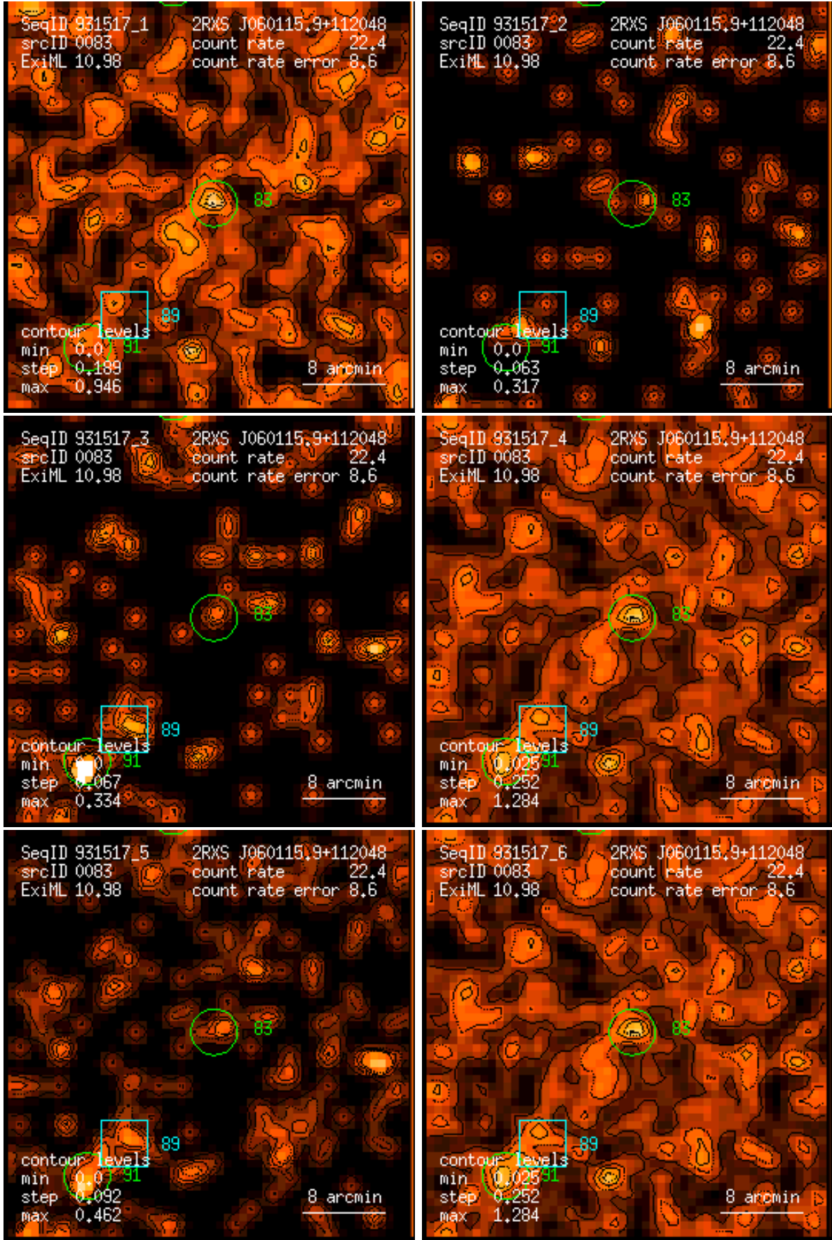
Figure 83: RASS 931517: detection 0083: band rate images, Gaussian filter: (1) PSPC channels 11 – 41, (2) 52 – 90, (3) 91 – 201, (4) 11 – 235, (5) 52 – 201, (6) 11 – 201. Broad band rates in counts/ks. Band rate contour levels in counts/ks/arcmin 2 .
