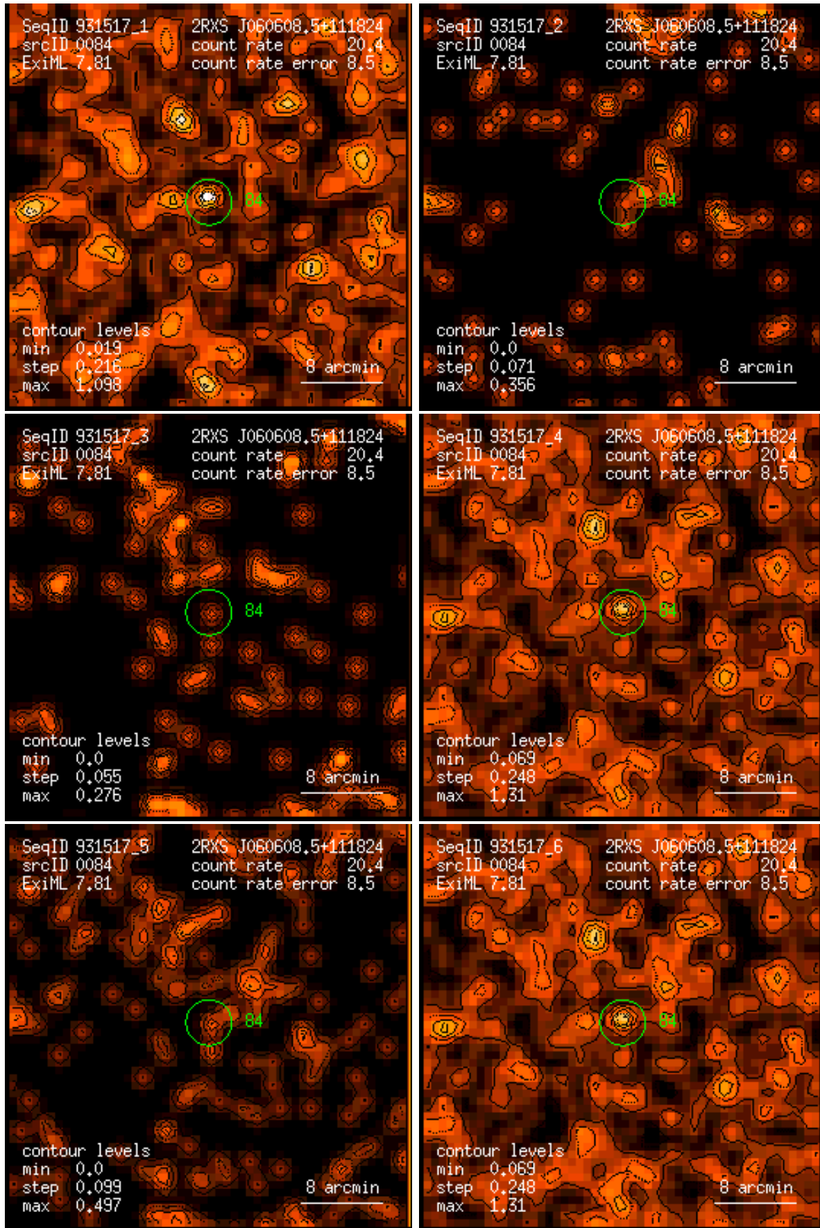
Figure 84: RASS 931517: detection 0084: band rate images, Gaussian filter: (1) PSPC channels 11 – 41, (2) 52 – 90, (3) 91 – 201, (4) 11 – 235, (5) 52 – 201, (6) 11 – 201. Broad band rates in counts/ks. Band rate contour levels in counts/ks/arcmin 2 .
