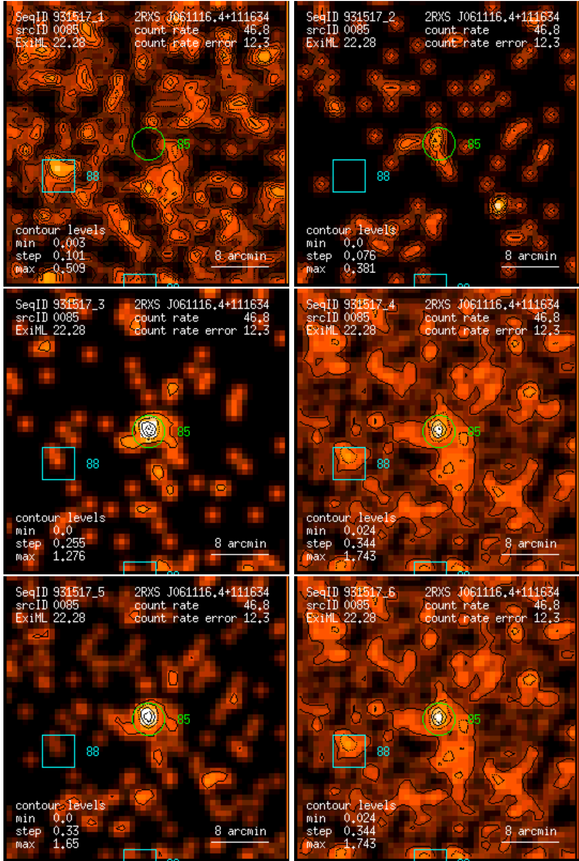
Figure 85: RASS 931517: detection 0085: band rate images, Gaussian filter: (1) PSPC channels 11 – 41, (2) 52 – 90, (3) 91 – 201, (4) 11 – 235, (5) 52 – 201, (6) 11 – 201. Broad band rates in counts/ks. Band rate contour levels in counts/ks/arcmin 2 .
