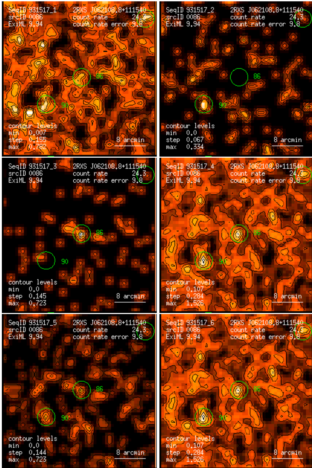
Figure 86: RASS 931517: detection 0086: band rate images, Gaussian filter: (1) PSPC channels 11 – 41, (2) 52 – 90, (3) 91 – 201, (4) 11 – 235, (5) 52 – 201, (6) 11 – 201. Broad band rates in counts/ks. Band rate contour levels in counts/ks/arcmin 2 .
