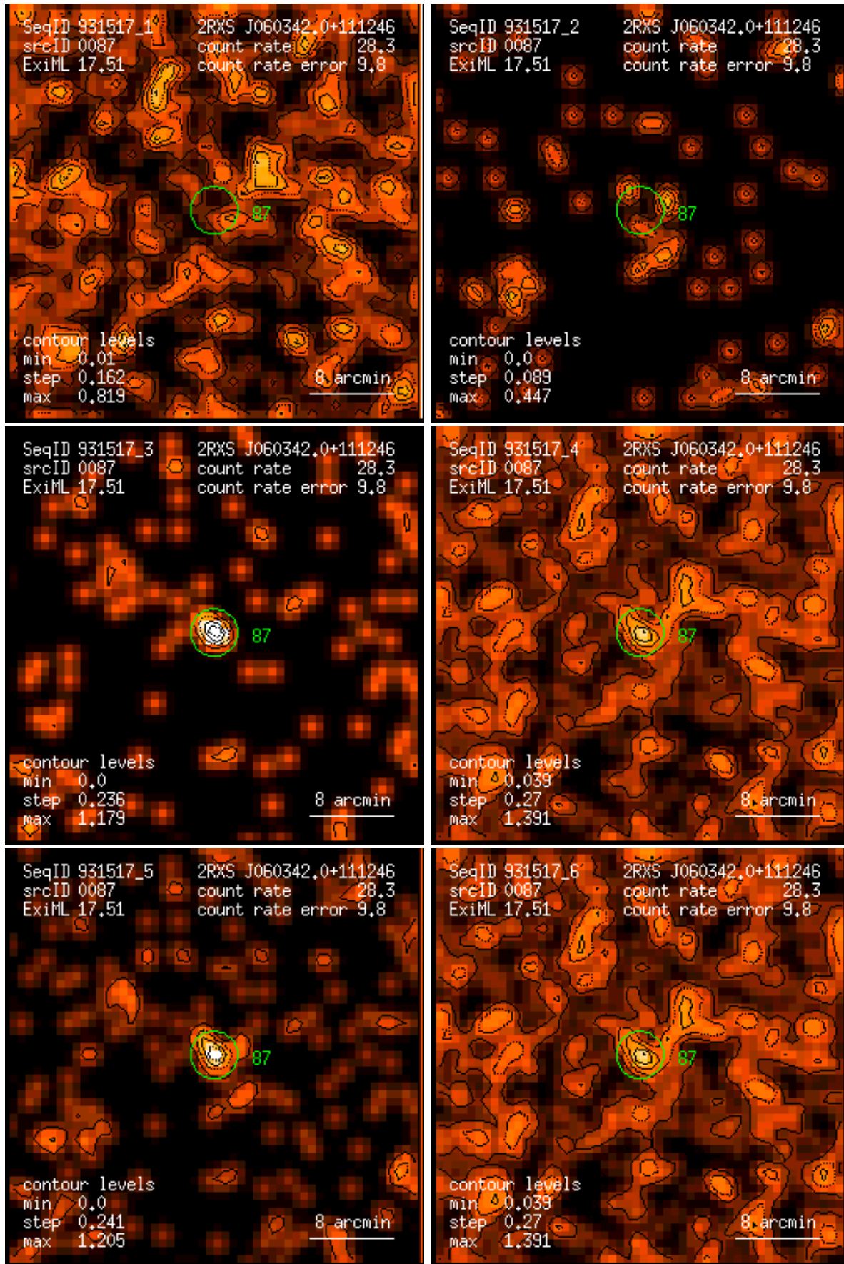
Figure 87: RASS 931517: detection 0087: band rate images, Gaussian filter: (1) PSPC channels 11 – 41, (2) 52 – 90, (3) 91 – 201, (4) 11 – 235, (5) 52 – 201, (6) 11 – 201. Broad band rates in counts/ks. Band rate contour levels in counts/ks/arcmin 2 .
