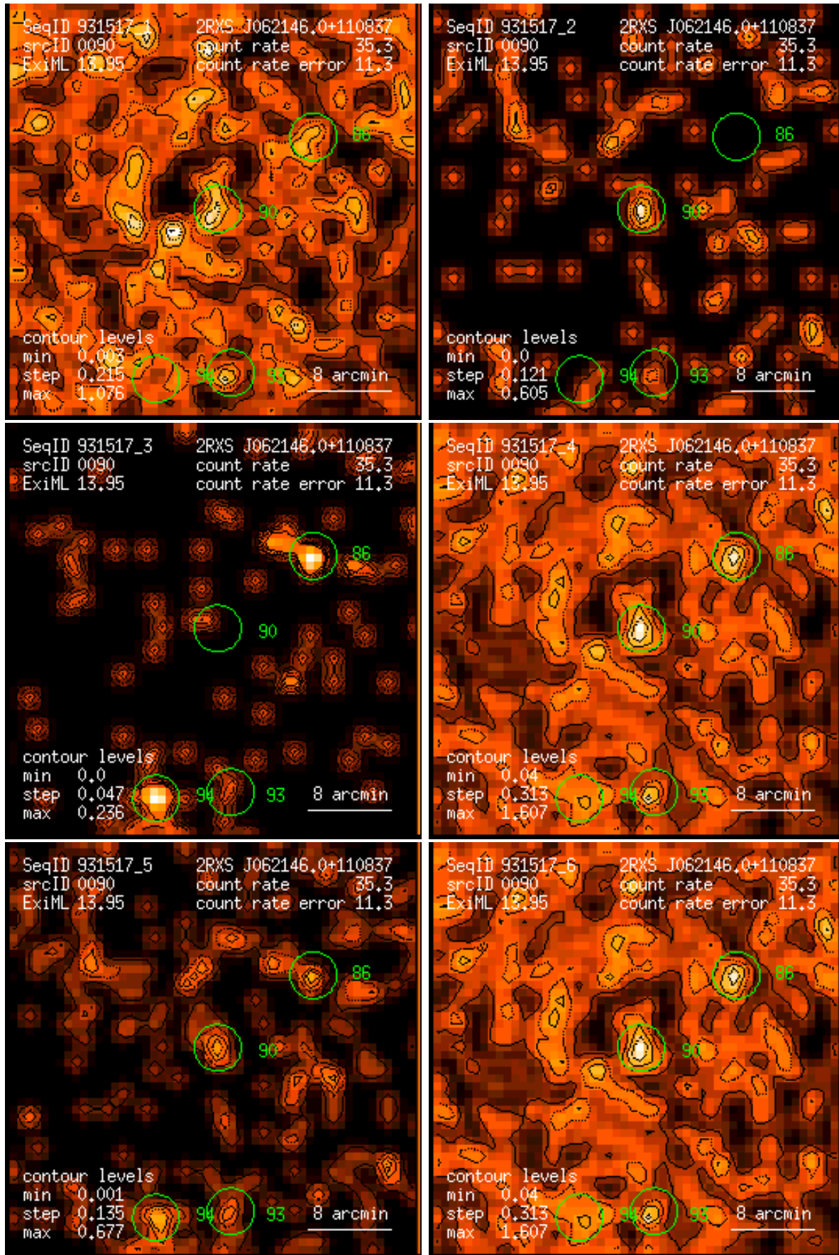
Figure 90: RASS 931517: detection 0090: band rate images, Gaussian filter: (1) PSPC channels 11 – 41, (2) 52 – 90, (3) 91 – 201, (4) 11 – 235, (5) 52 – 201, (6) 11 – 201. Broad band rates in counts/ks. Band rate contour levels in counts/ks/arcmin 2 .
