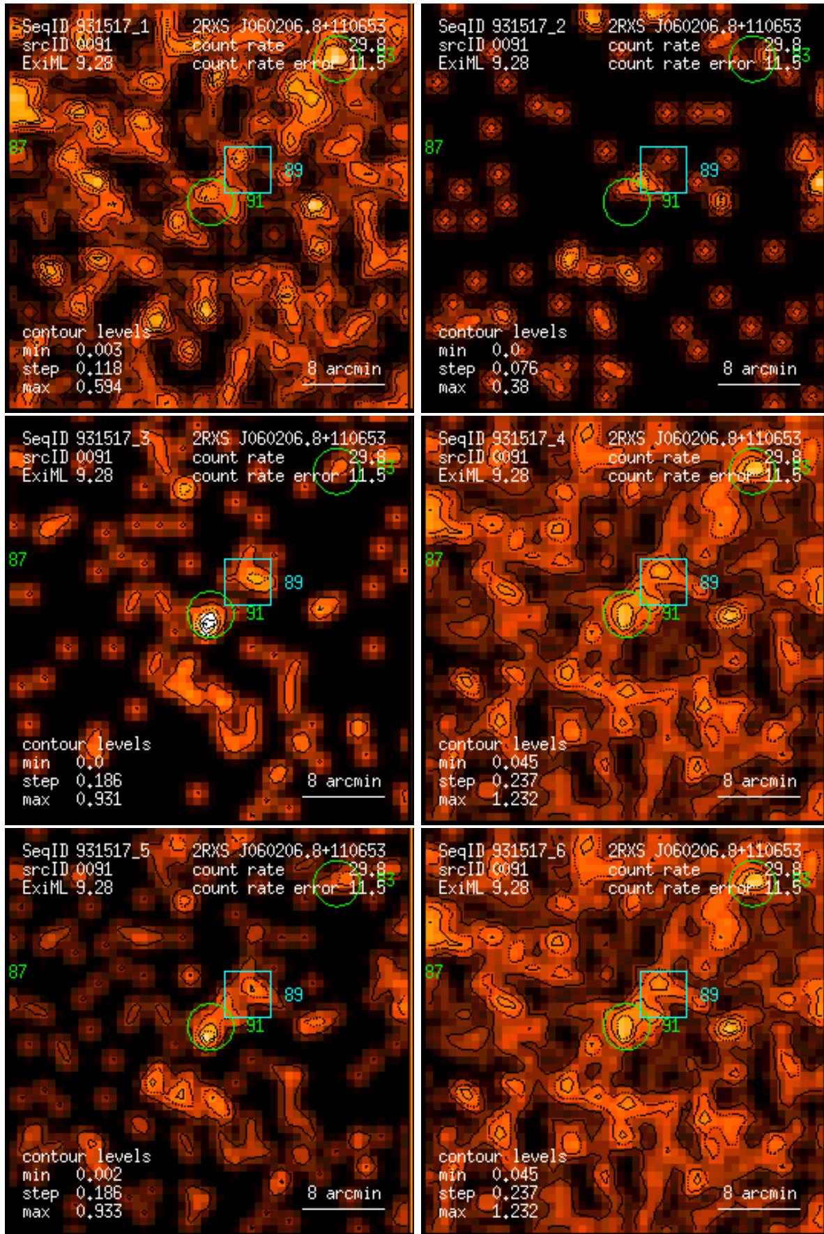
Figure 91: RASS 931517: detection 0091: band rate images, Gaussian filter: (1) PSPC channels 11 – 41, (2) 52 – 90, (3) 91 – 201, (4) 11 – 235, (5) 52 – 201, (6) 11 – 201. Broad band rates in counts/ks. Band rate contour levels in counts/ks/arcmin 2 .
