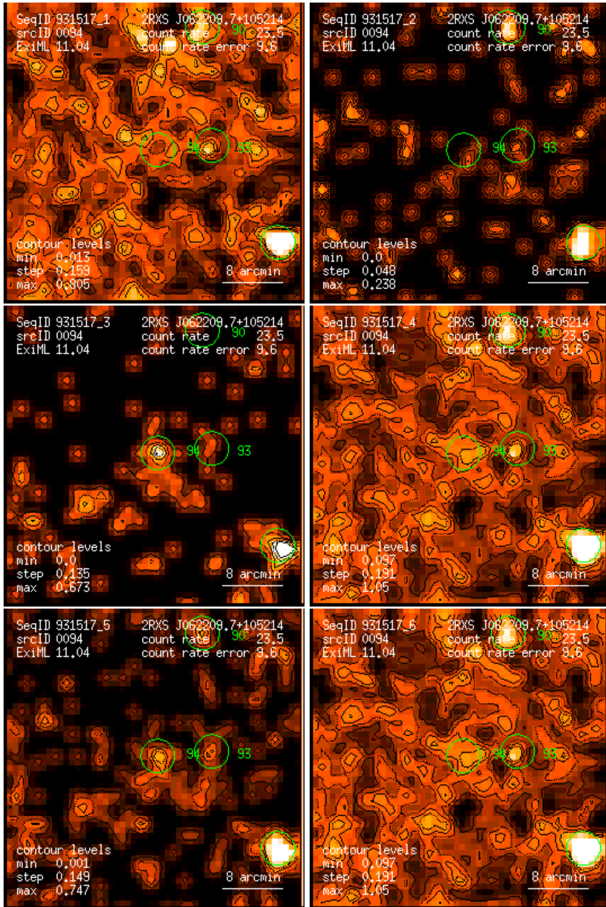
Figure 94: RASS 931517: detection 0094: band rate images, Gaussian filter: (1) PSPC channels 11 – 41, (2) 52 – 90, (3) 91 – 201, (4) 11 – 235, (5) 52 – 201, (6) 11 – 201. Broad band rates in counts/ks. Band rate contour levels in counts/ks/arcmin 2 .
