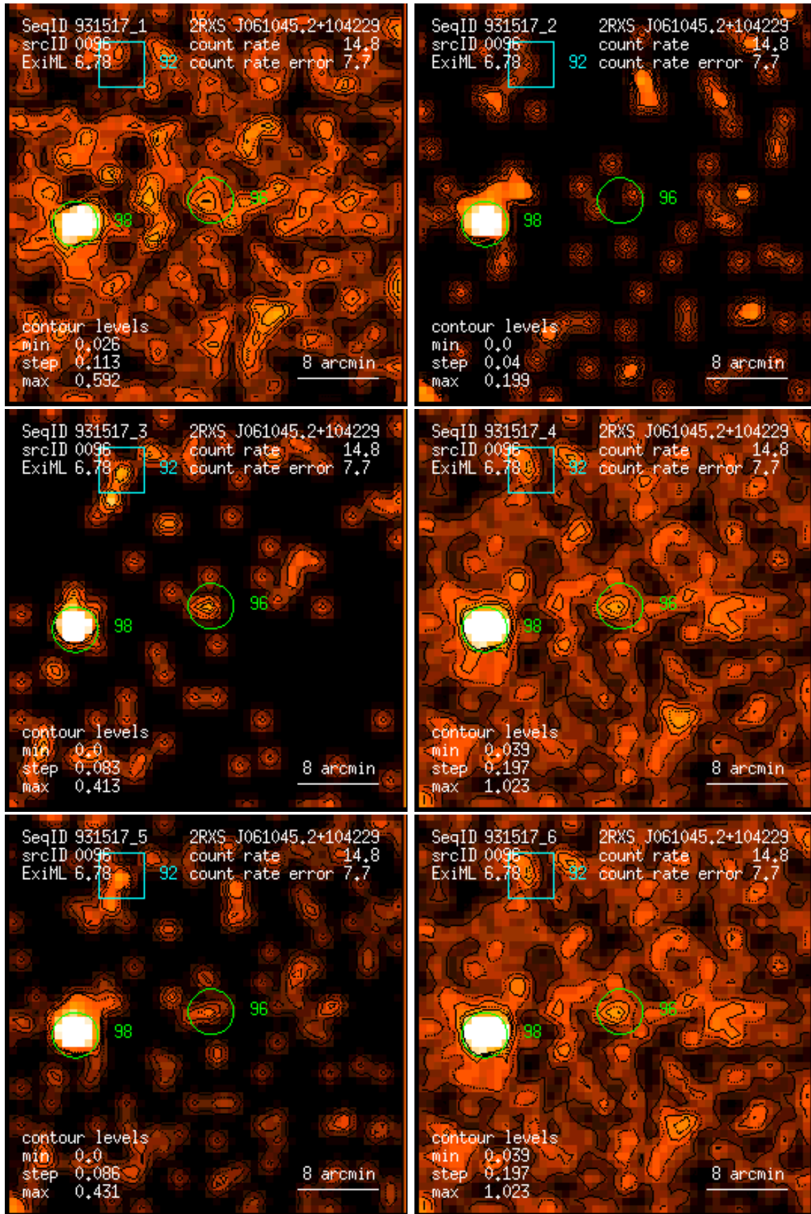
Figure 96: RASS 931517: detection 0096: band rate images, Gaussian filter: (1) PSPC channels 11 – 41, (2) 52 – 90, (3) 91 – 201, (4) 11 – 235, (5) 52 – 201, (6) 11 – 201. Broad band rates in counts/ks. Band rate contour levels in counts/ks/arcmin 2 .
