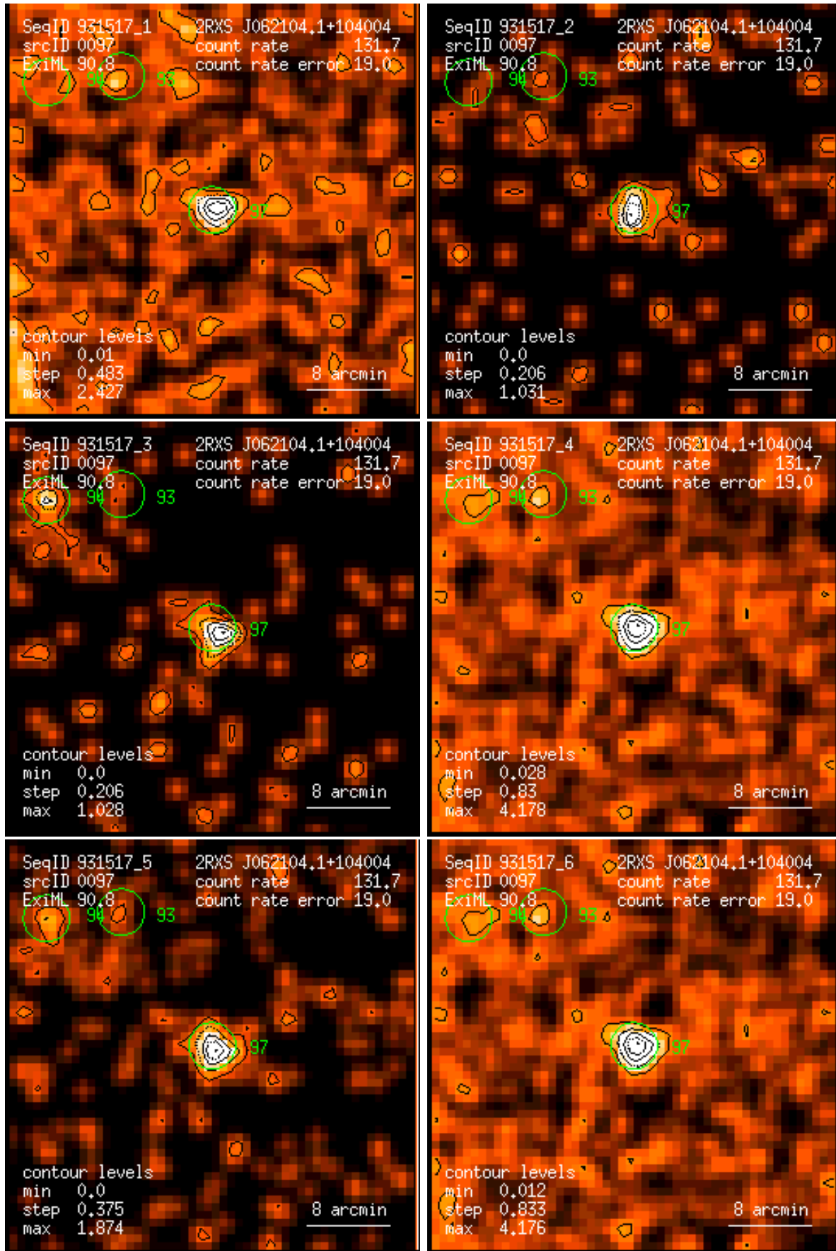
Figure 97: RASS 931517: detection 0097: band rate images, Gaussian filter: (1) PSPC channels 11 – 41, (2) 52 – 90, (3) 91 – 201, (4) 11 – 235, (5) 52 – 201, (6) 11 – 201. Broad band rates in counts/ks. Band rate contour levels in counts/ks/arcmin 2 .
